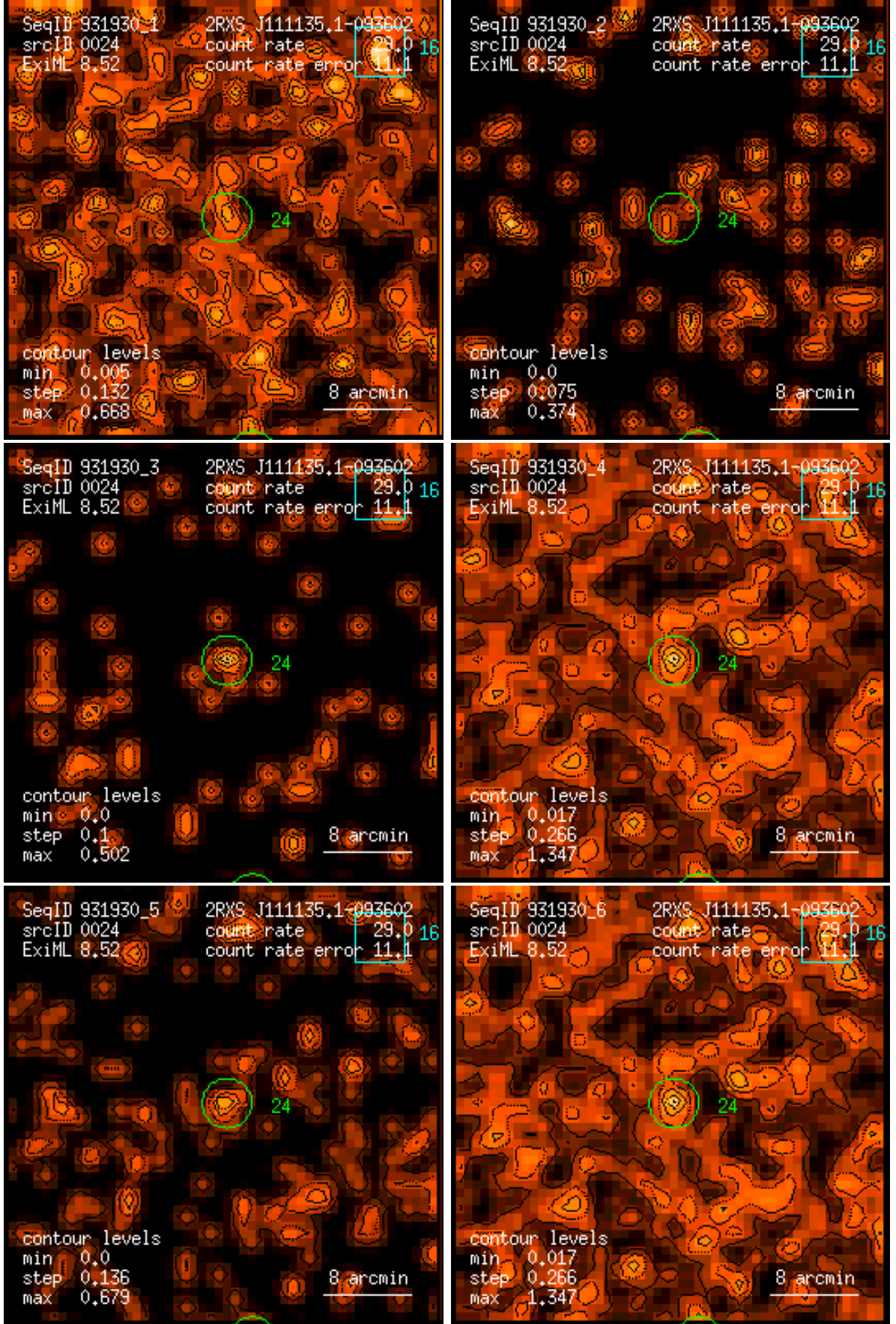
Figure 24: RASS 931930: detection 0024: band rate images, Gaussian filter: (1) PSPC channels 11 – 41, (2) 52 – 90, (3) 91 – 201, (4) 11 – 235, (5) 52 – 201, (6) 11 – 201. Broad band rates in counts/ks. Band rate contour levels in counts/ks/arcmin 2 .
