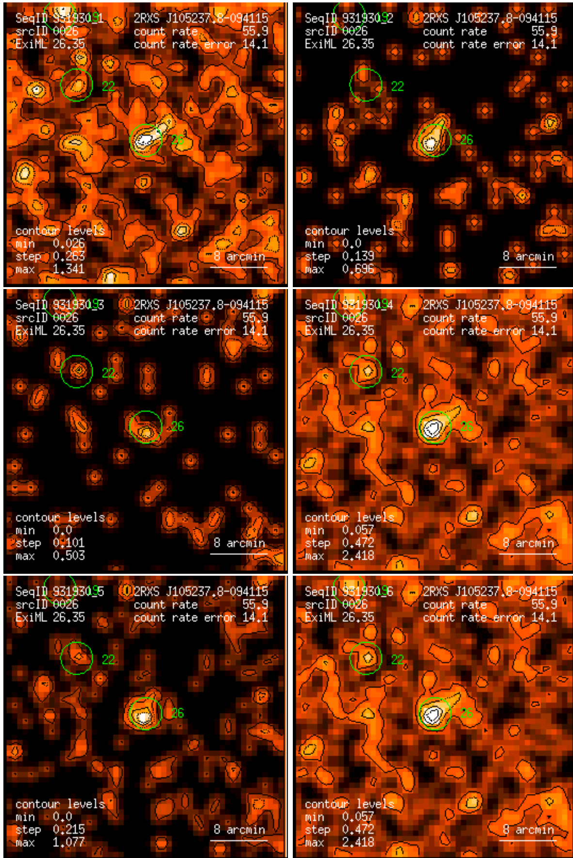
Figure 26: RASS 931930: detection 0026: band rate images, Gaussian filter: (1) PSPC channels 11 – 41, (2) 52 – 90, (3) 91 – 201, (4) 11 – 235, (5) 52 – 201, (6) 11 – 201. Broad band rates in counts/ks. Band rate contour levels in counts/ks/arcmin 2 .
