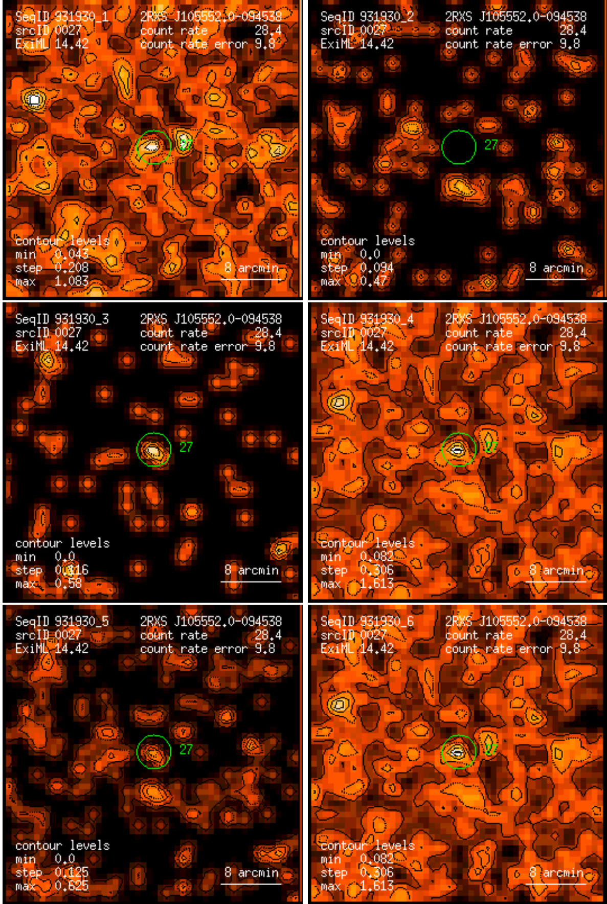
Figure 27: RASS 931930: detection 0027: band rate images, Gaussian filter: (1) PSPC channels 11 – 41, (2) 52 – 90, (3) 91 – 201, (4) 11 – 235, (5) 52 – 201, (6) 11 – 201. Broad band rates in counts/ks. Band rate contour levels in counts/ks/arcmin 2 .
