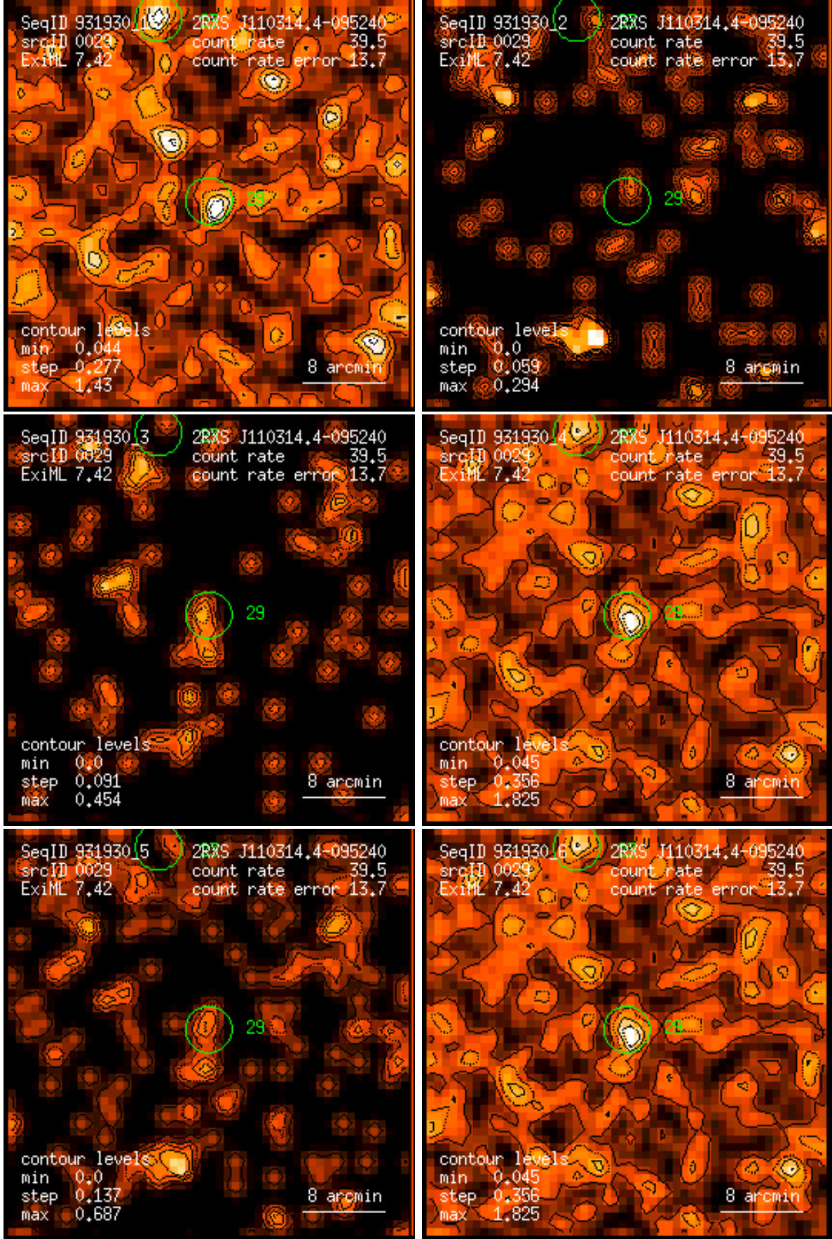
Figure 29: RASS 931930: detection 0029: band rate images, Gaussian filter: (1) PSPC channels 11 – 41, (2) 52 – 90, (3) 91 – 201, (4) 11 – 235, (5) 52 – 201, (6) 11 – 201. Broad band rates in counts/ks. Band rate contour levels in counts/ks/arcmin 2 .
