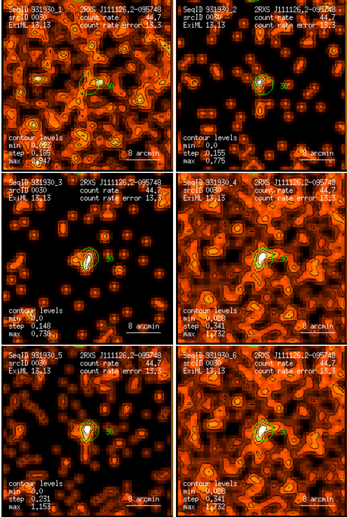
Figure 30: RASS 931930: detection 0030: band rate images, Gaussian filter: (1) PSPC channels 11 – 41, (2) 52 – 90, (3) 91 – 201, (4) 11 – 235, (5) 52 – 201, (6) 11 – 201. Broad band rates in counts/ks. Band rate contour levels in counts/ks/arcmin 2 .
