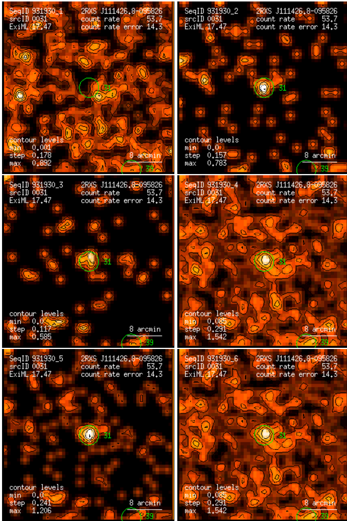
Figure 31: RASS 931930: detection 0031: band rate images, Gaussian filter: (1) PSPC channels 11 – 41, (2) 52 – 90, (3) 91 – 201, (4) 11 – 235, (5) 52 – 201, (6) 11 – 201. Broad band rates in counts/ks. Band rate contour levels in counts/ks/arcmin 2 .
