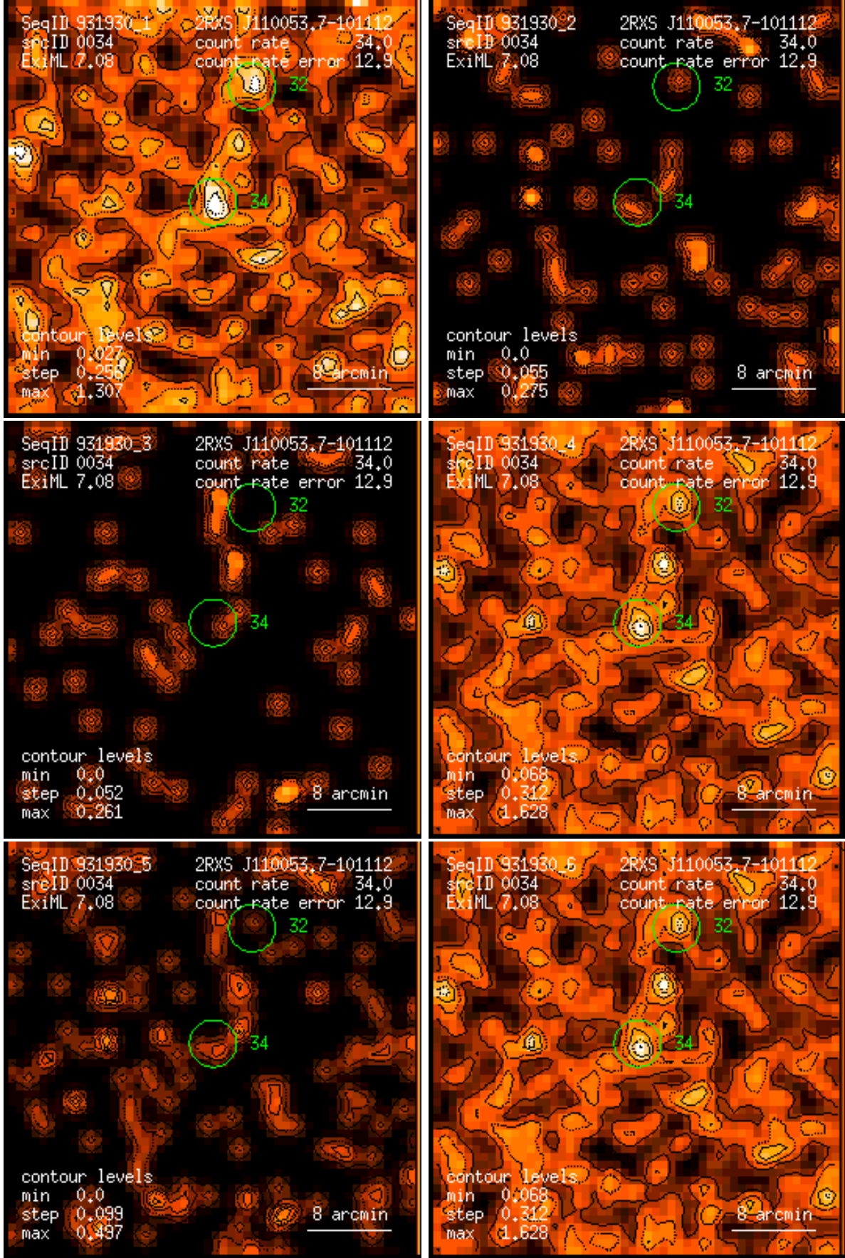
Figure 34: RASS 931930: detection 0034: band rate images, Gaussian filter: (1) PSPC channels 11 – 41, (2) 52 – 90, (3) 91 – 201, (4) 11 – 235, (5) 52 – 201, (6) 11 – 201. Broad band rates in counts/ks. Band rate contour levels in counts/ks/arcmin 2 .
