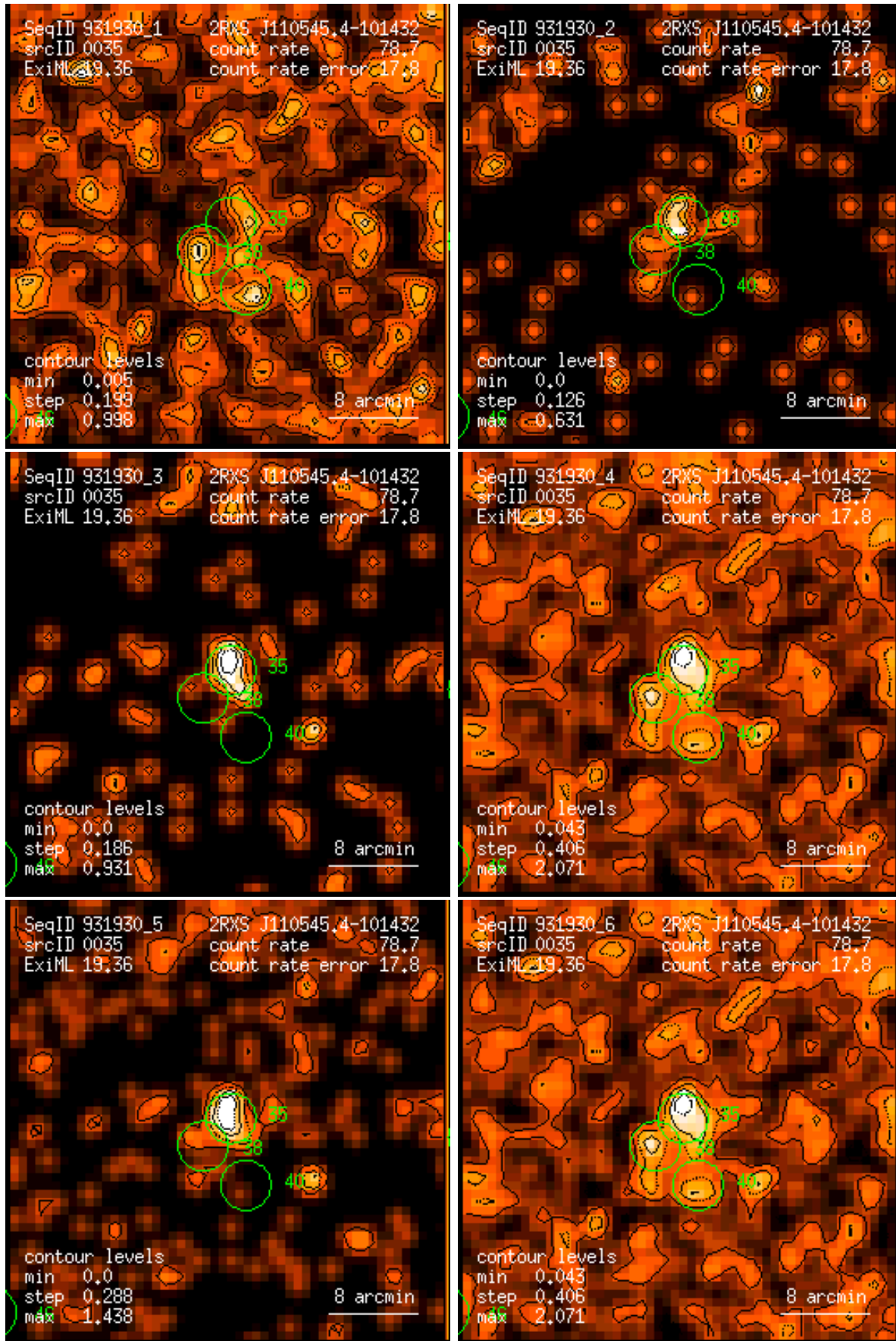
Figure 35: RASS 931930: detection 0035: band rate images, Gaussian filter: (1) PSPC channels 11 – 41, (2) 52 – 90, (3) 91 – 201, (4) 11 – 235, (5) 52 – 201, (6) 11 – 201. Broad band rates in counts/ks. Band rate contour levels in counts/ks/arcmin 2 .
