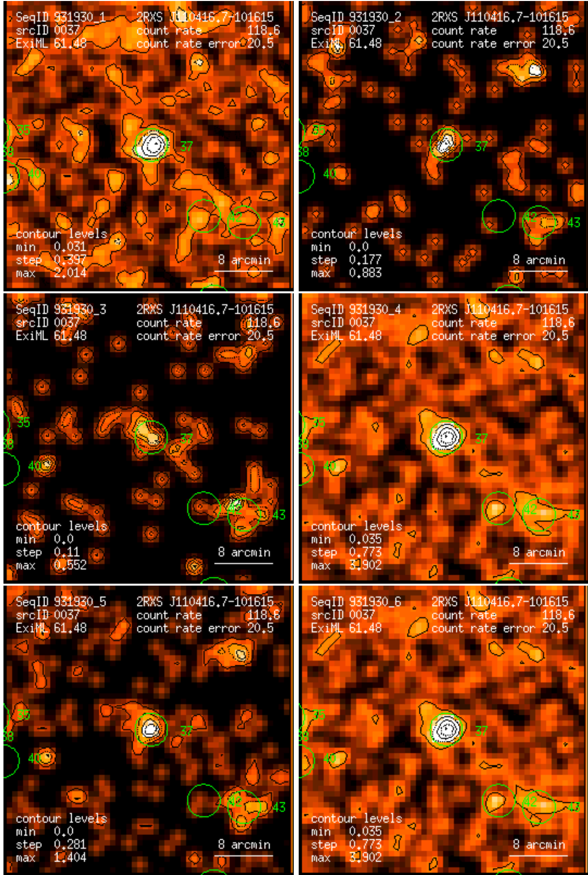
Figure 37: RASS 931930: detection 0037: band rate images, Gaussian filter: (1) PSPC channels 11 – 41, (2) 52 – 90, (3) 91 – 201, (4) 11 – 235, (5) 52 – 201, (6) 11 – 201. Broad band rates in counts/ks. Band rate contour levels in counts/ks/arcmin 2 .
