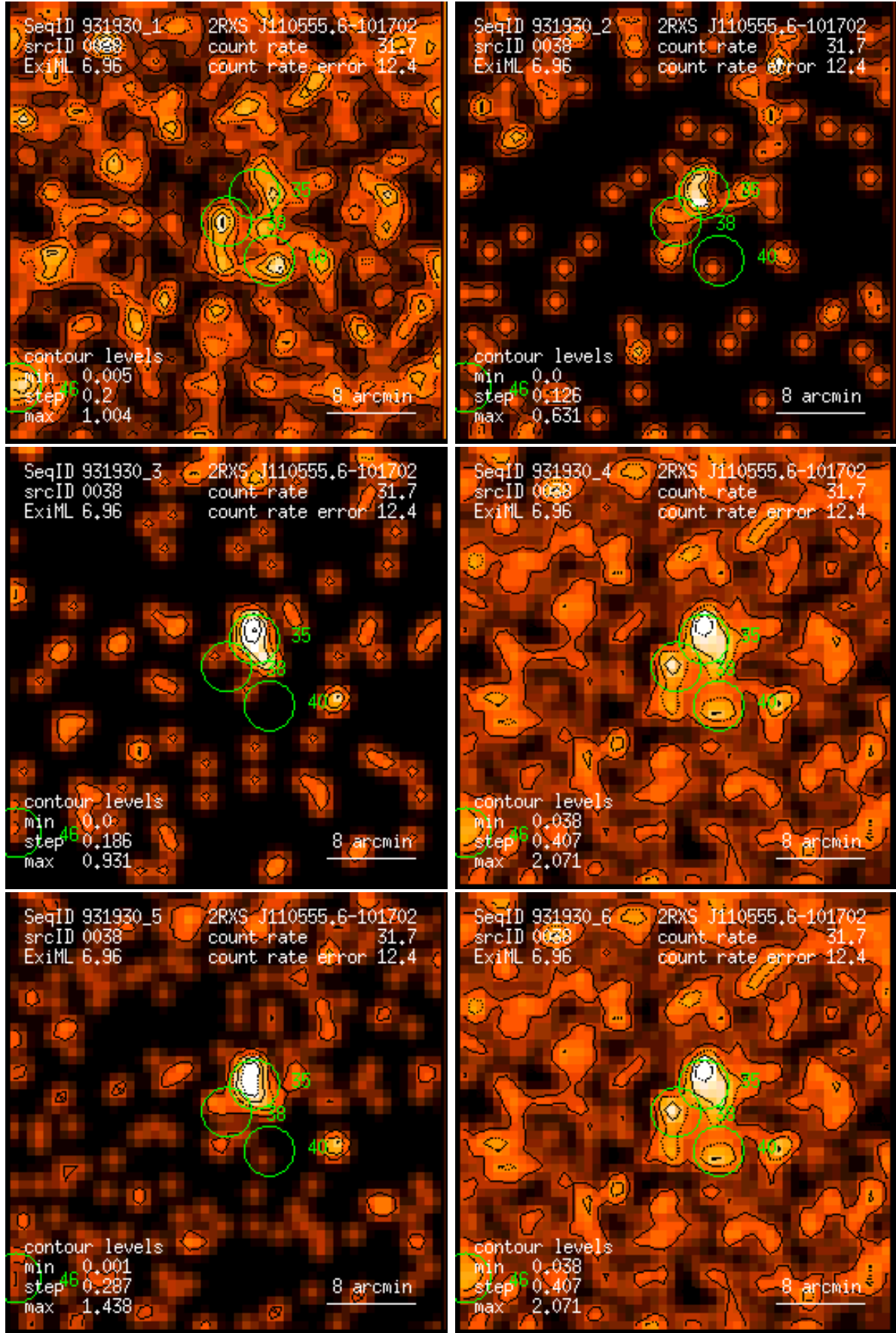
Figure 38: RASS 931930: detection 0038: band rate images, Gaussian filter: (1) PSPC channels 11 – 41, (2) 52 – 90, (3) 91 – 201, (4) 11 – 235, (5) 52 – 201, (6) 11 – 201. Broad band rates in counts/ks. Band rate contour levels in counts/ks/arcmin 2 .
