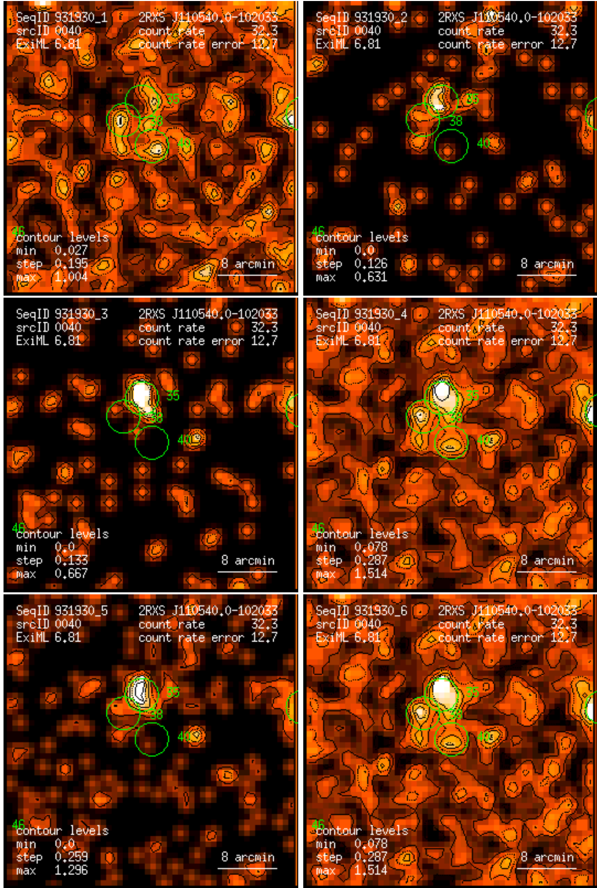
Figure 40: RASS 931930: detection 0040: band rate images, Gaussian filter: (1) PSPC channels 11 – 41, (2) 52 – 90, (3) 91 – 201, (4) 11 – 235, (5) 52 – 201, (6) 11 – 201. Broad band rates in counts/ks. Band rate contour levels in counts/ks/arcmin 2 .
