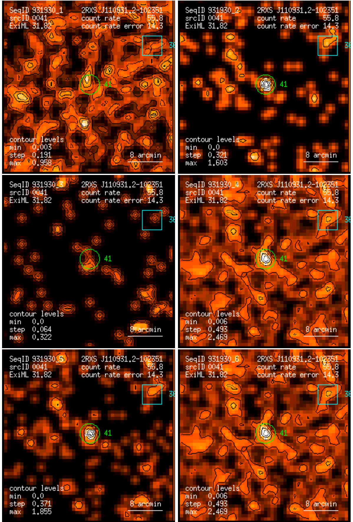
Figure 41: RASS 931930: detection 0041: band rate images, Gaussian filter: (1) PSPC channels 11 – 41, (2) 52 – 90, (3) 91 – 201, (4) 11 – 235, (5) 52 – 201, (6) 11 – 201. Broad band rates in counts/ks. Band rate contour levels in counts/ks/arcmin 2 .
