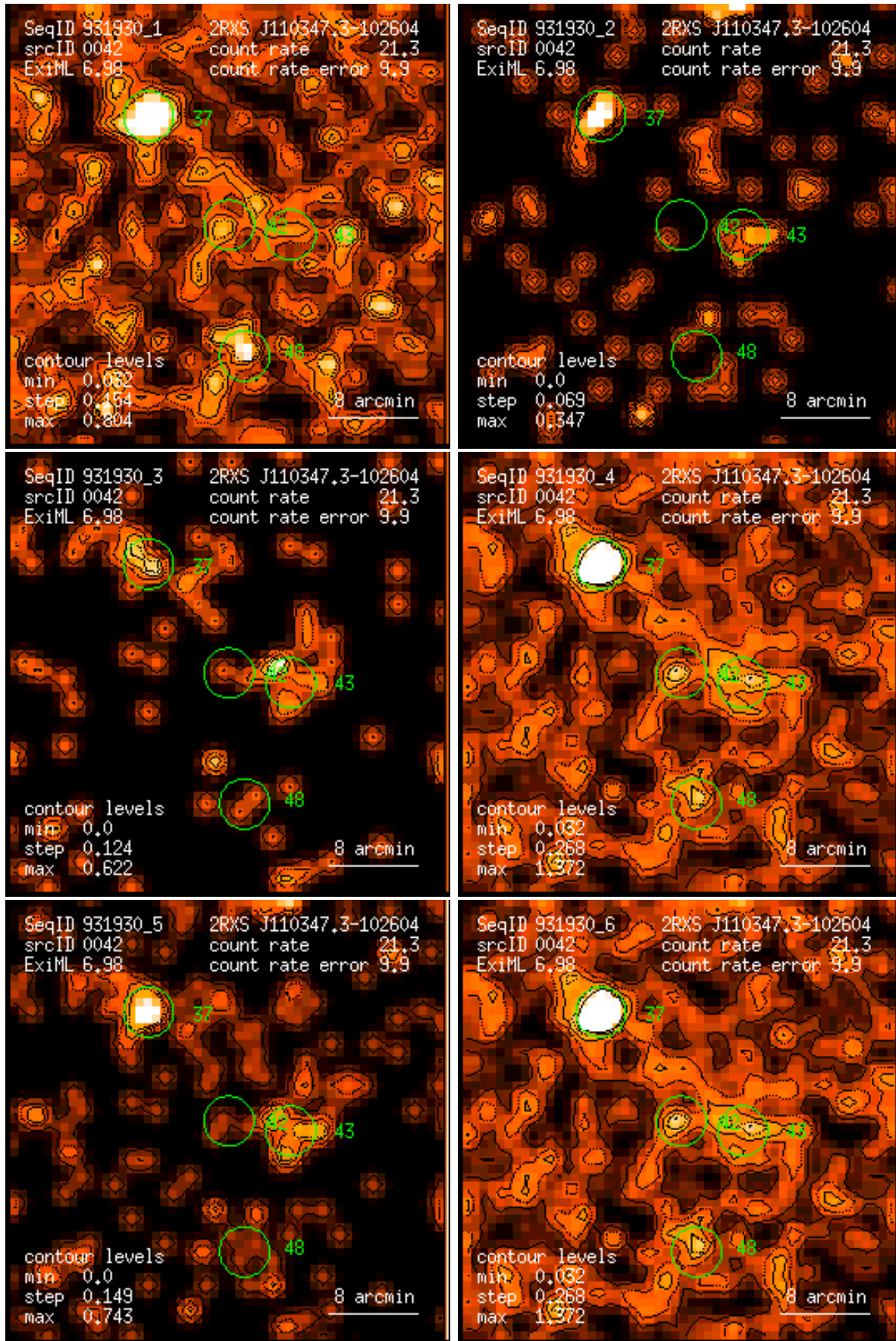
Figure 42: RASS 931930: detection 0042: band rate images, Gaussian filter: (1) PSPC channels 11 – 41, (2) 52 – 90, (3) 91 – 201, (4) 11 – 235, (5) 52 – 201, (6) 11 – 201. Broad band rates in counts/ks. Band rate contour levels in counts/ks/arcmin 2 .
