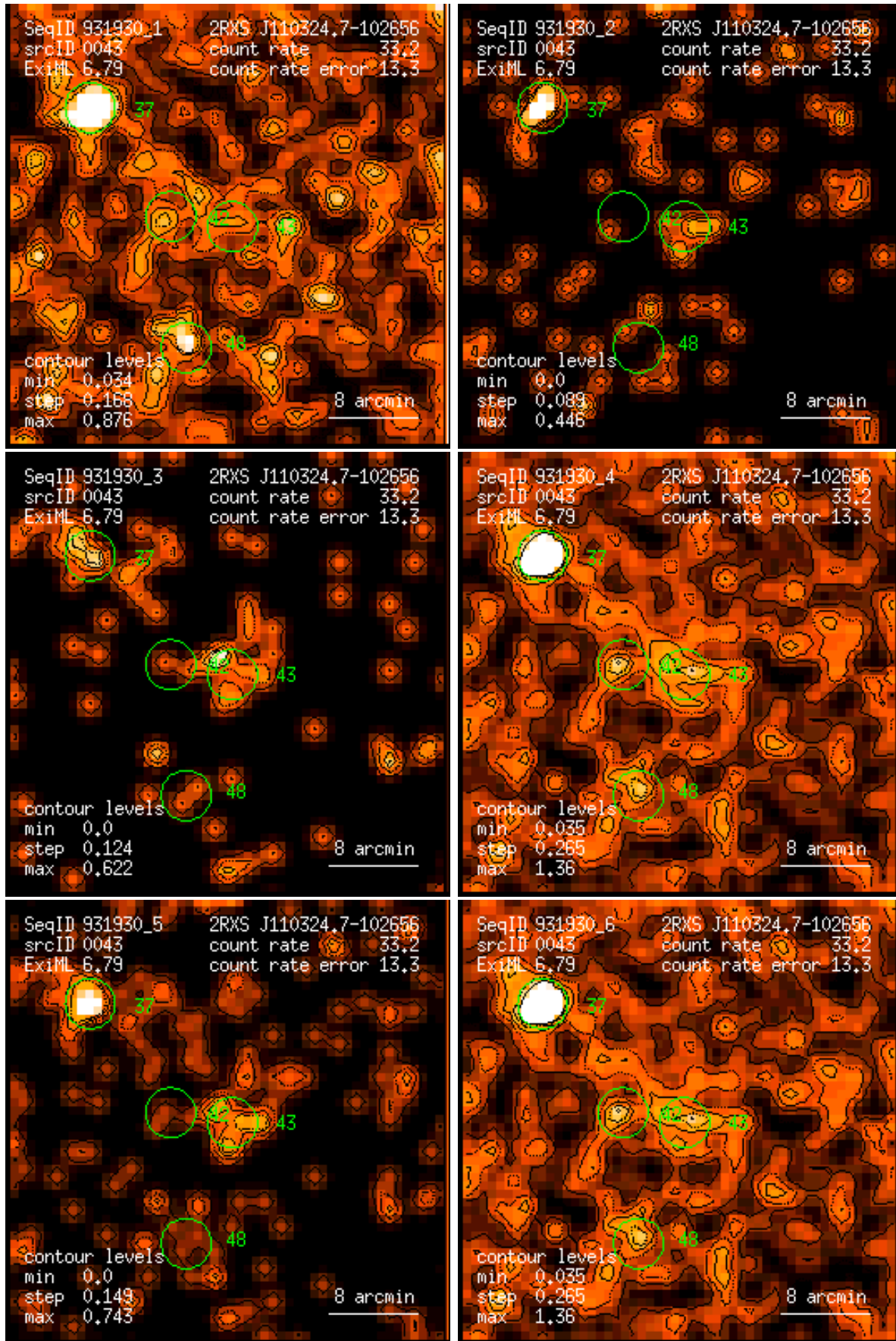
Figure 43: RASS 931930: detection 0043: band rate images, Gaussian filter: (1) PSPC channels 11 – 41, (2) 52 – 90, (3) 91 – 201, (4) 11 – 235, (5) 52 – 201, (6) 11 – 201. Broad band rates in counts/ks. Band rate contour levels in counts/ks/arcmin 2 .
