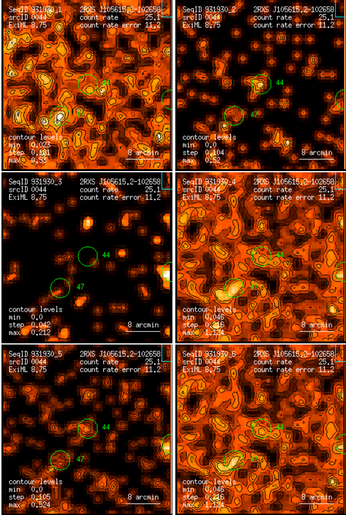
Figure 44: RASS 931930: detection 0044: band rate images, Gaussian filter: (1) PSPC channels 11 – 41, (2) 52 – 90, (3) 91 – 201, (4) 11 – 235, (5) 52 – 201, (6) 11 – 201. Broad band rates in counts/ks. Band rate contour levels in counts/ks/arcmin 2 .
