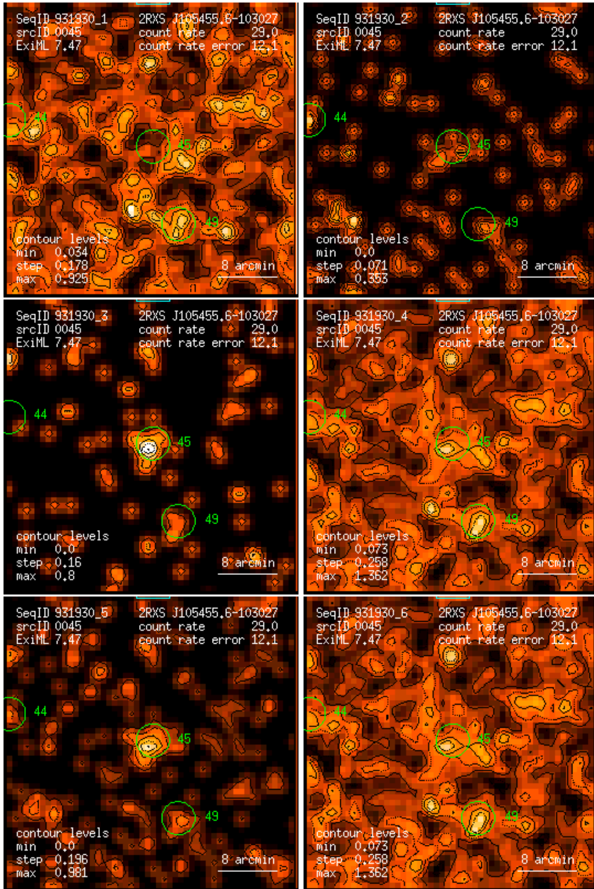
Figure 45: RASS 931930: detection 0045: band rate images, Gaussian filter: (1) PSPC channels 11 – 41, (2) 52 – 90, (3) 91 – 201, (4) 11 – 235, (5) 52 – 201, (6) 11 – 201. Broad band rates in counts/ks. Band rate contour levels in counts/ks/arcmin 2 .
