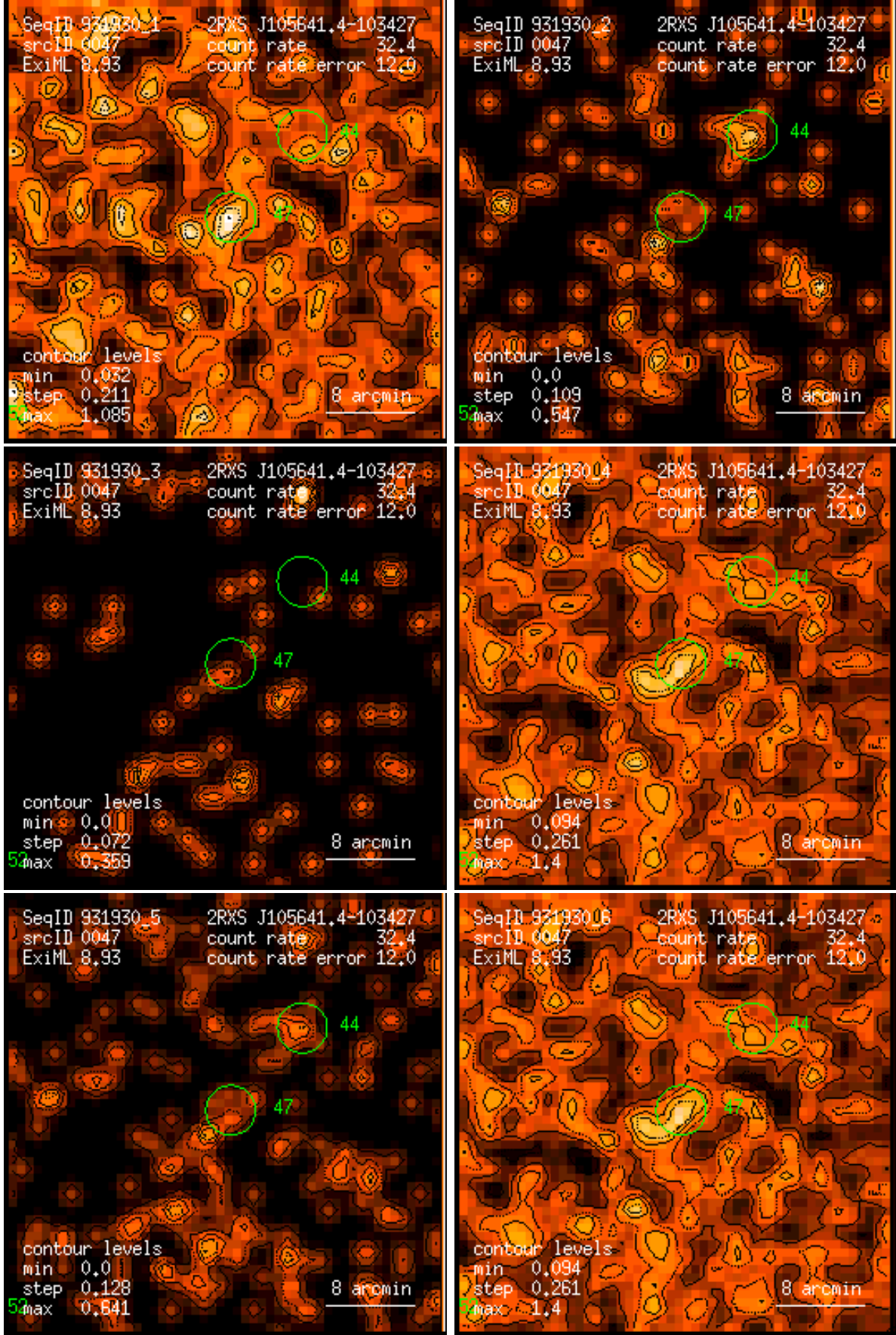
Figure 47: RASS 931930: detection 0047: band rate images, Gaussian filter: (1) PSPC channels 11 – 41, (2) 52 – 90, (3) 91 – 201, (4) 11 – 235, (5) 52 – 201, (6) 11 – 201. Broad band rates in counts/ks. Band rate contour levels in counts/ks/arcmin 2 .
