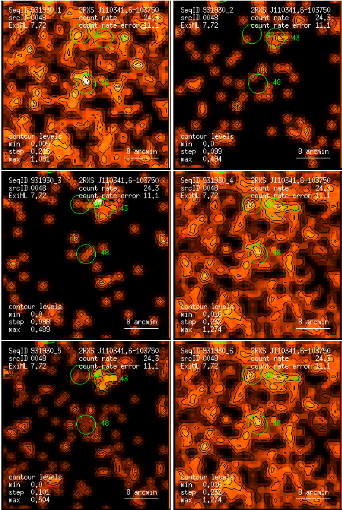
Figure 48: RASS 931930: detection 0048: band rate images, Gaussian filter: (1) PSPC channels 11 – 41, (2) 52 – 90, (3) 91 – 201, (4) 11 – 235, (5) 52 – 201, (6) 11 – 201. Broad band rates in counts/ks. Band rate contour levels in counts/ks/arcmin 2 .
