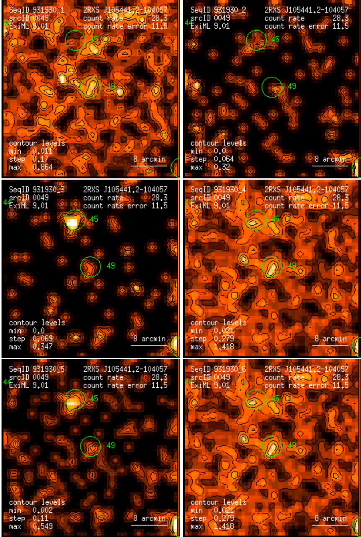
Figure 49: RASS 931930: detection 0049: band rate images, Gaussian filter: (1) PSPC channels 11 – 41, (2) 52 – 90, (3) 91 – 201, (4) 11 – 235, (5) 52 – 201, (6) 11 – 201. Broad band rates in counts/ks. Band rate contour levels in counts/ks/arcmin 2 .
