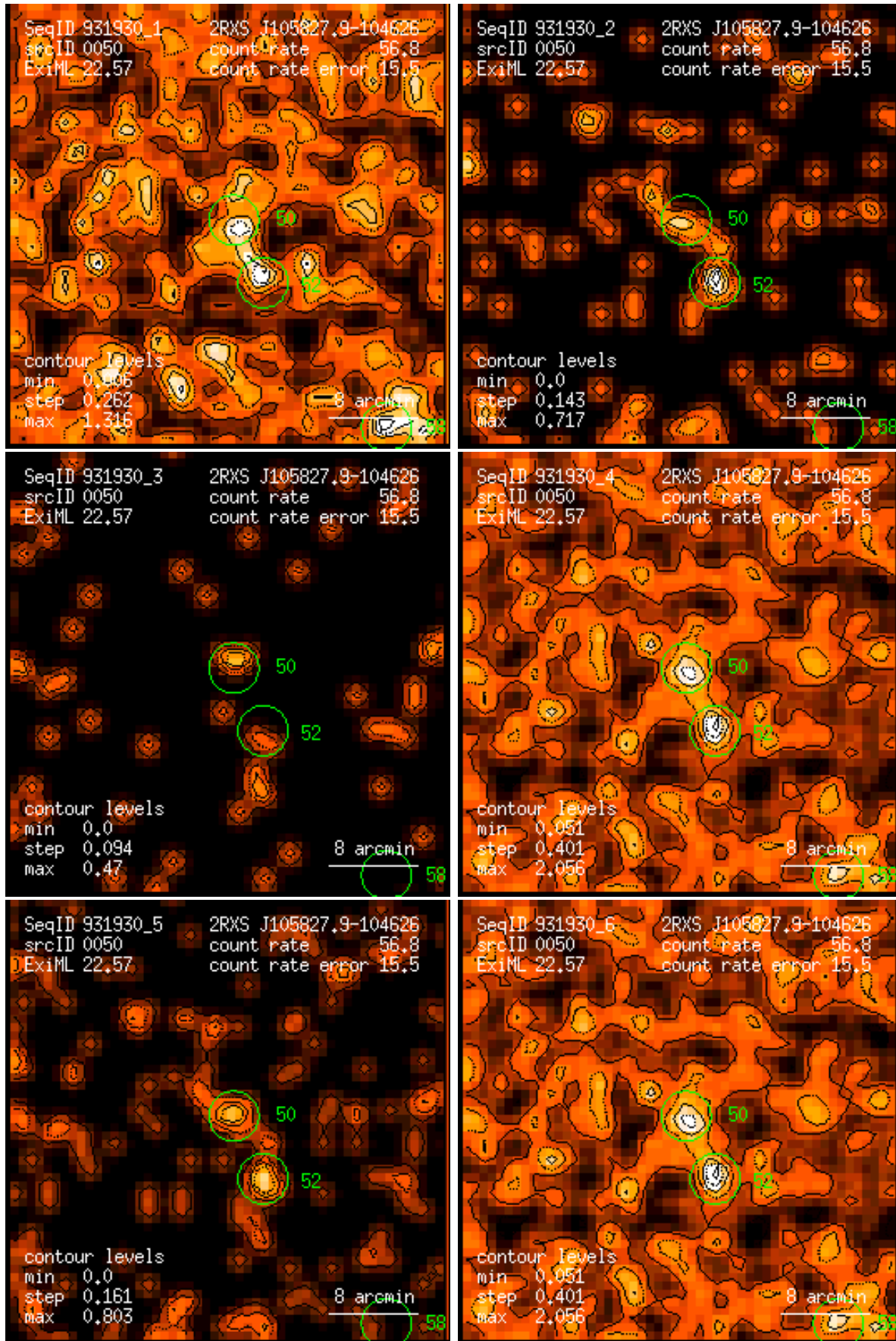
Figure 50: RASS 931930: detection 0050: band rate images, Gaussian filter: (1) PSPC channels 11 – 41, (2) 52 – 90, (3) 91 – 201, (4) 11 – 235, (5) 52 – 201, (6) 11 – 201. Broad band rates in counts/ks. Band rate contour levels in counts/ks/arcmin 2 .
