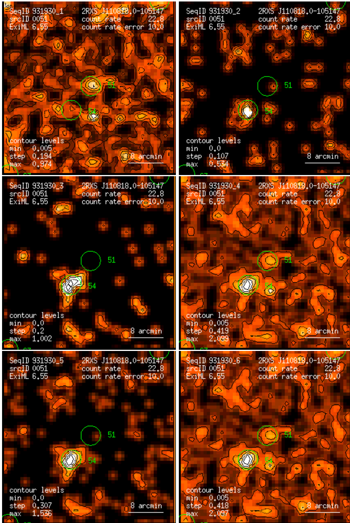
Figure 51: RASS 931930: detection 0051: band rate images, Gaussian filter: (1) PSPC channels 11 – 41, (2) 52 – 90, (3) 91 – 201, (4) 11 – 235, (5) 52 – 201, (6) 11 – 201. Broad band rates in counts/ks. Band rate contour levels in counts/ks/arcmin 2 .
