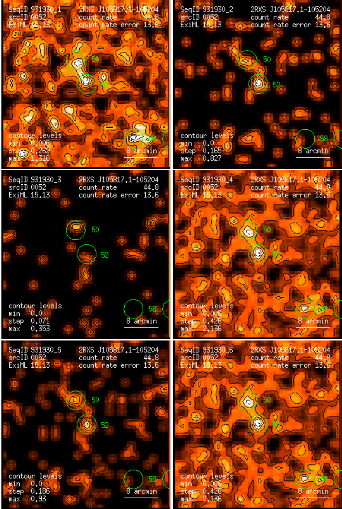
Figure 52: RASS 931930: detection 0052: band rate images, Gaussian filter: (1) PSPC channels 11 – 41, (2) 52 – 90, (3) 91 – 201, (4) 11 – 235, (5) 52 – 201, (6) 11 – 201. Broad band rates in counts/ks. Band rate contour levels in counts/ks/arcmin 2 .
