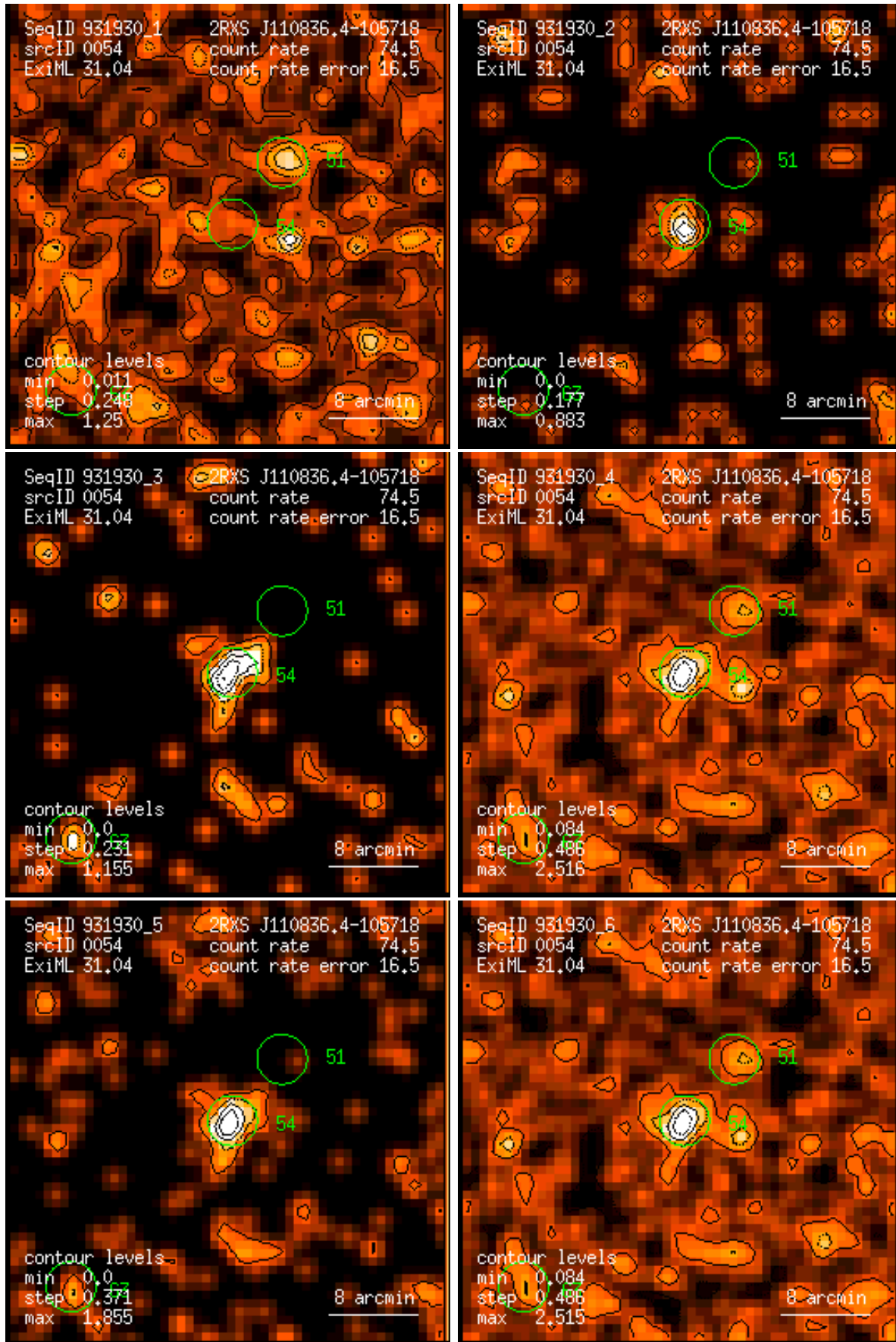
Figure 54: RASS 931930: detection 0054: band rate images, Gaussian filter: (1) PSPC channels 11 – 41, (2) 52 – 90, (3) 91 – 201, (4) 11 – 235, (5) 52 – 201, (6) 11 – 201. Broad band rates in counts/ks. Band rate contour levels in counts/ks/arcmin 2 .
