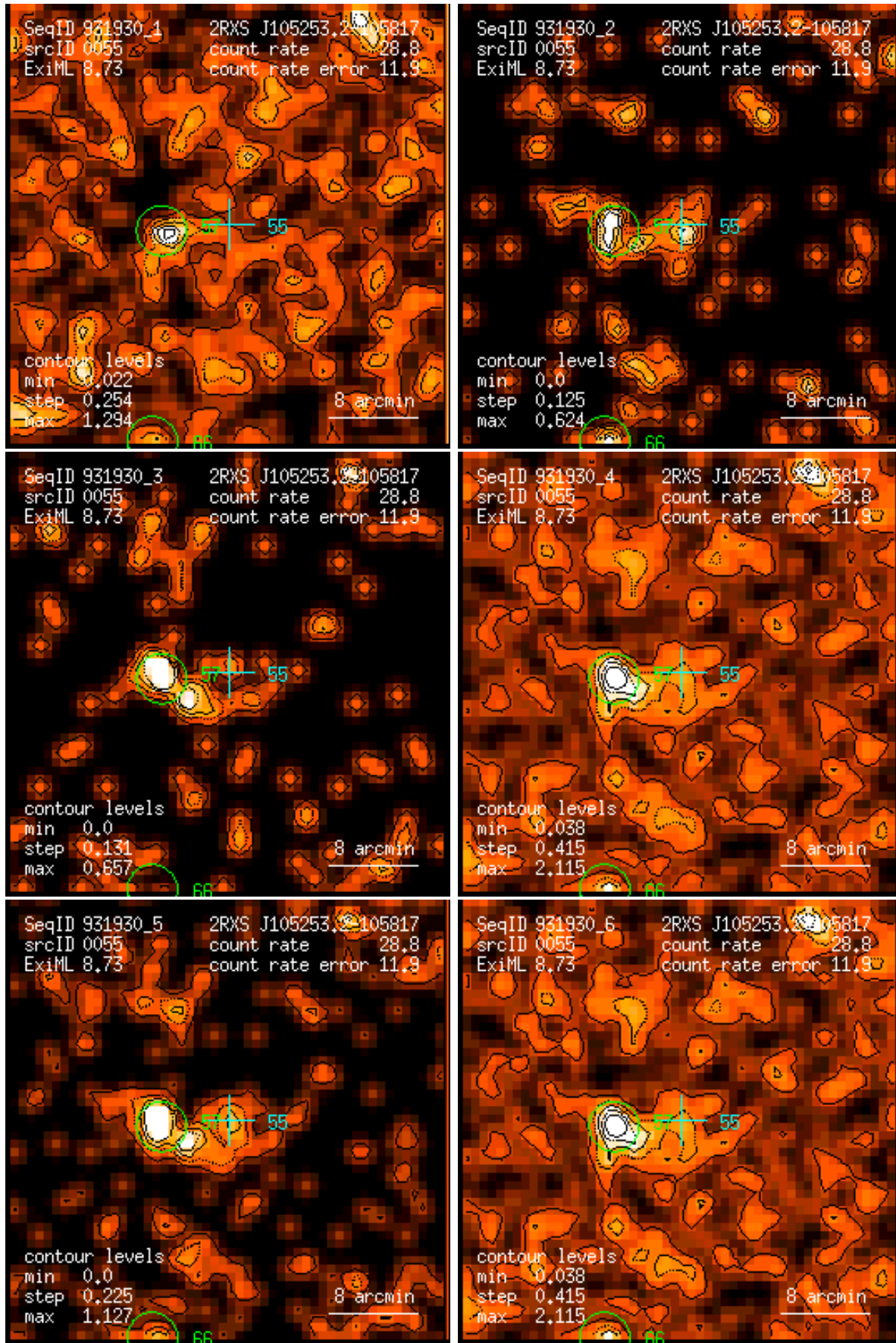
Figure 55: RASS 931930: detection 0055: band rate images, Gaussian filter: (1) PSPC channels 11 – 41, (2) 52 – 90, (3) 91 – 201, (4) 11 – 235, (5) 52 – 201, (6) 11 – 201. Broad band rates in counts/ks. Band rate contour levels in counts/ks/arcmin 2 .
