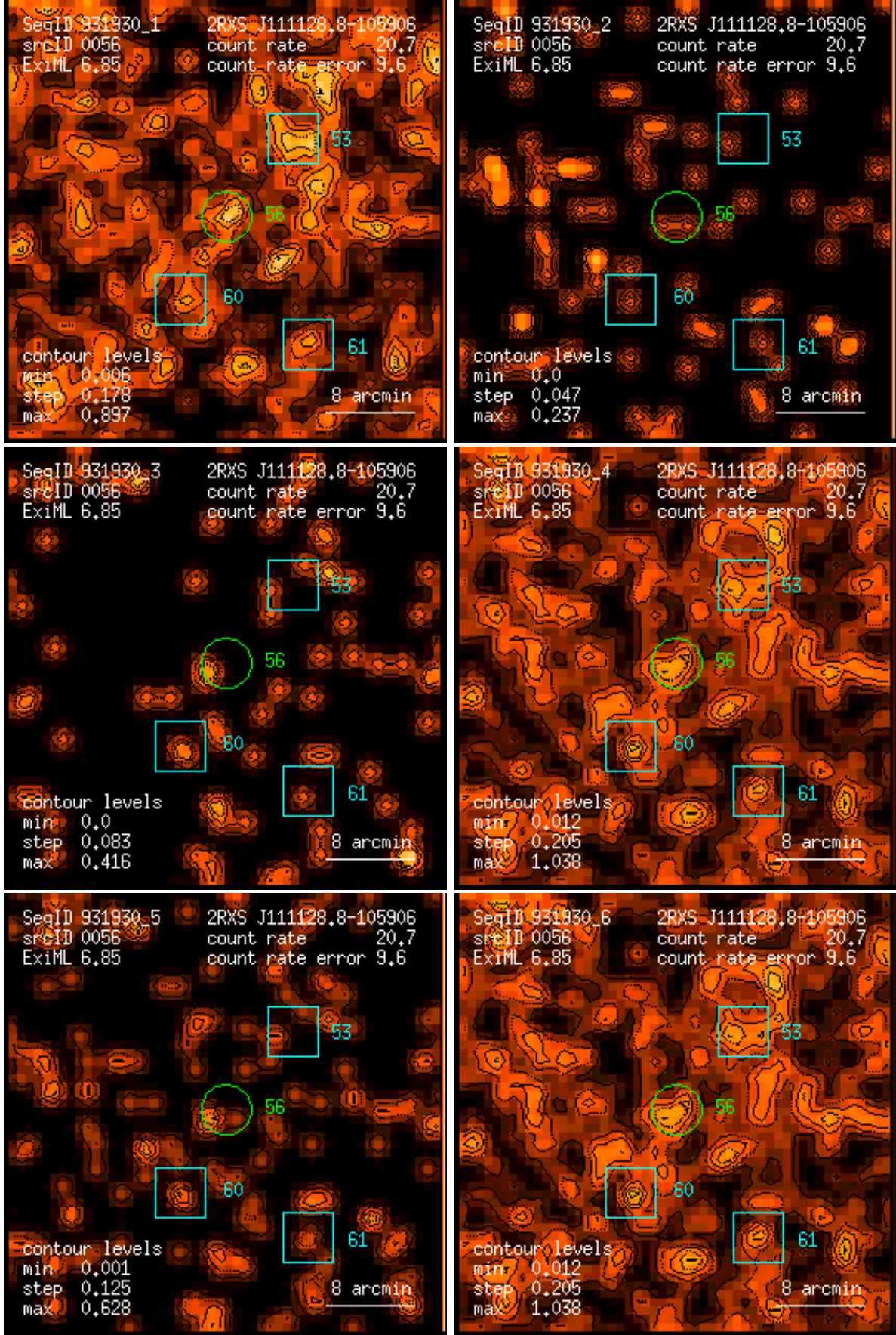
Figure 56: RASS 931930: detection 0056: band rate images, Gaussian filter: (1) PSPC channels 11 – 41, (2) 52 – 90, (3) 91 – 201, (4) 11 – 235, (5) 52 – 201, (6) 11 – 201. Broad band rates in counts/ks. Band rate contour levels in counts/ks/arcmin 2 .
