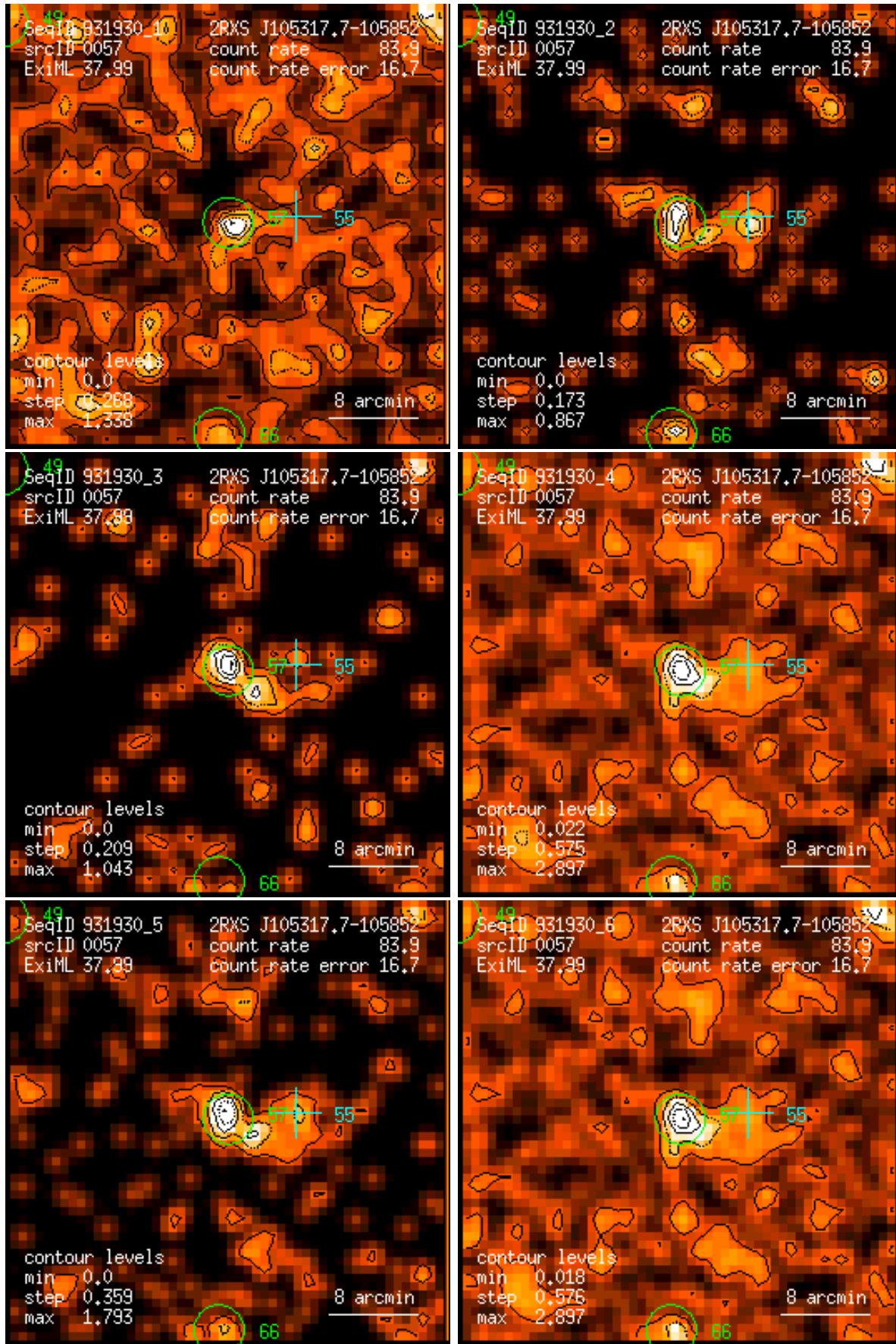
Figure 57: RASS 931930: detection 0057: band rate images, Gaussian filter: (1) PSPC channels 11 – 41, (2) 52 – 90, (3) 91 – 201, (4) 11 – 235, (5) 52 – 201, (6) 11 – 201. Broad band rates in counts/ks. Band rate contour levels in counts/ks/arcmin 2 .
