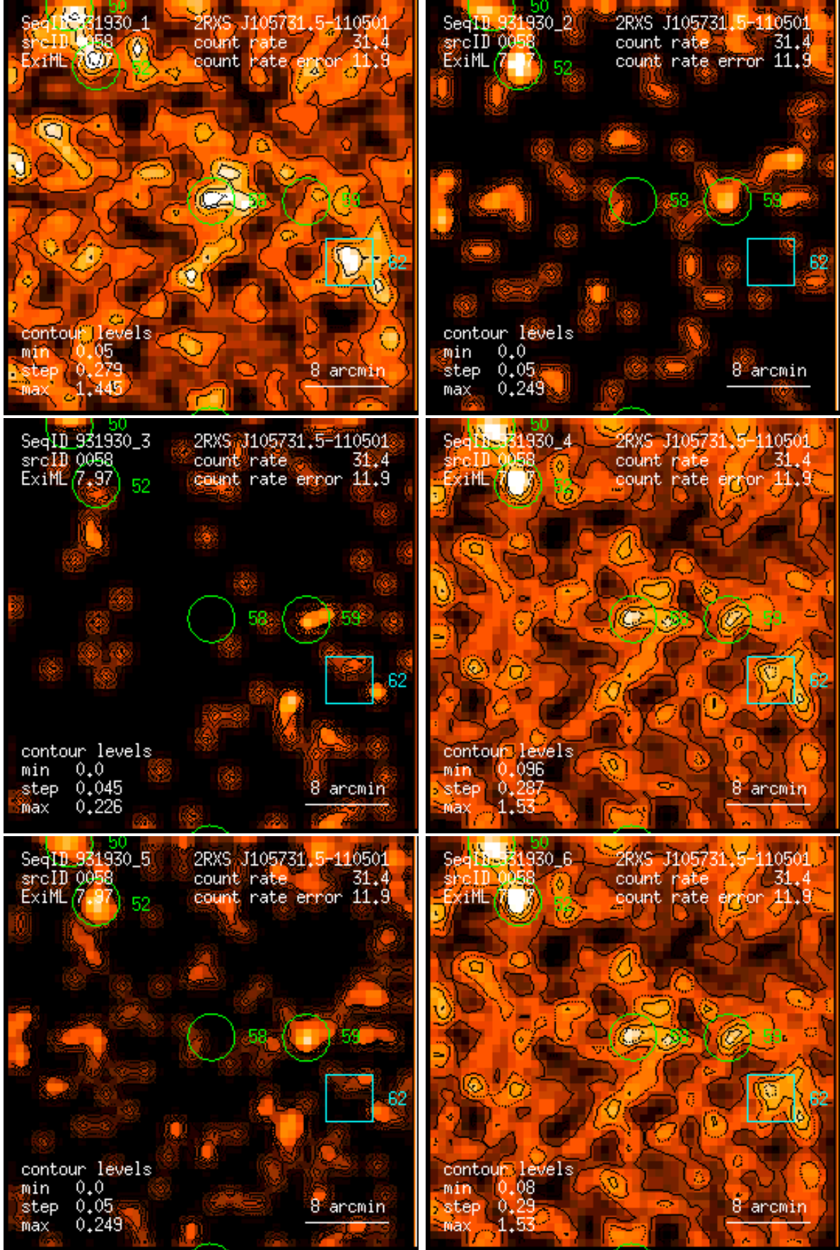
Figure 58: RASS 931930: detection 0058: band rate images, Gaussian filter: (1) PSPC channels 11 – 41, (2) 52 – 90, (3) 91 – 201, (4) 11 – 235, (5) 52 – 201, (6) 11 – 201. Broad band rates in counts/ks. Band rate contour levels in counts/ks/arcmin 2 .
