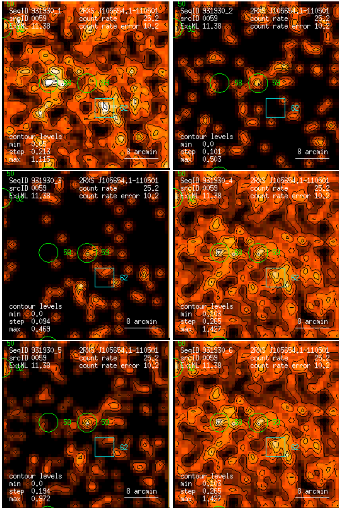
Figure 59: RASS 931930: detection 0059: band rate images, Gaussian filter: (1) PSPC channels 11 – 41, (2) 52 – 90, (3) 91 – 201, (4) 11 – 235, (5) 52 – 201, (6) 11 – 201. Broad band rates in counts/ks. Band rate contour levels in counts/ks/arcmin 2 .
