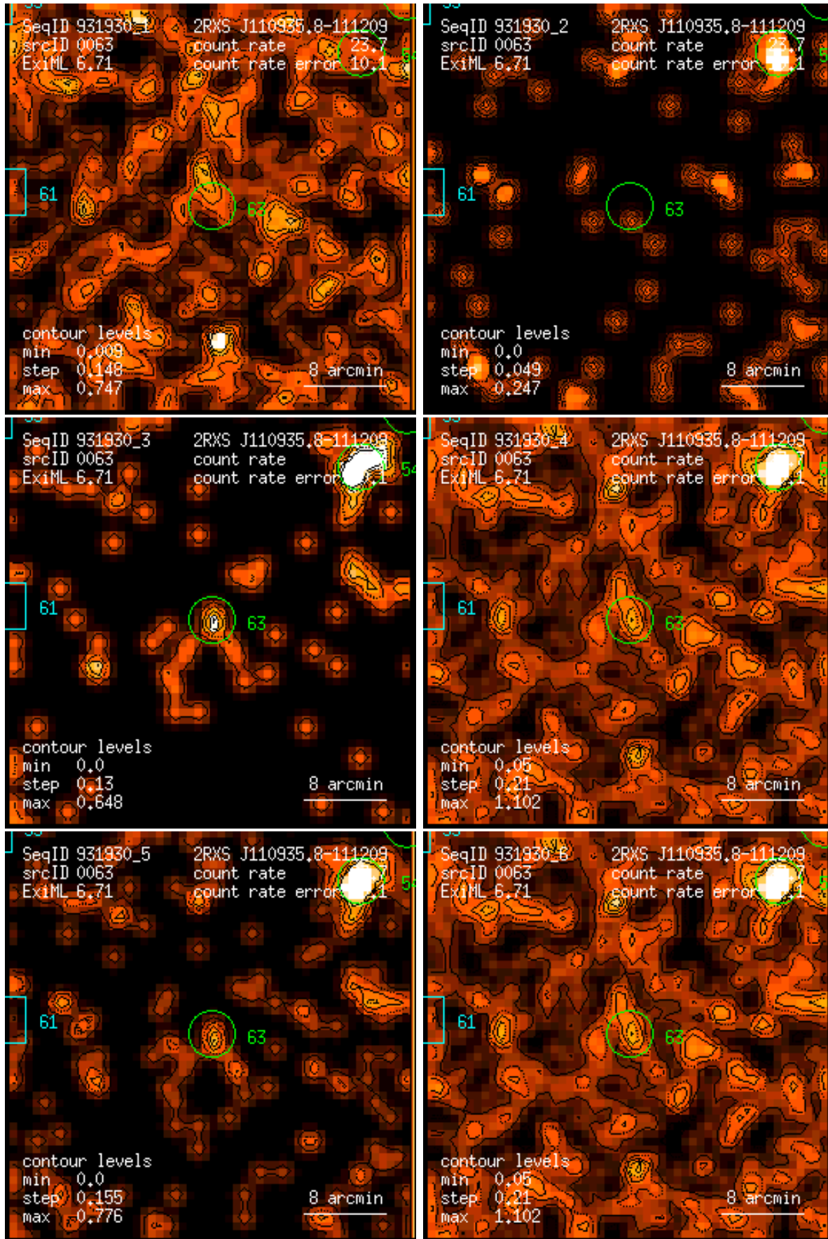
Figure 63: RASS 931930: detection 0063: band rate images, Gaussian filter: (1) PSPC channels 11 – 41, (2) 52 – 90, (3) 91 – 201, (4) 11 – 235, (5) 52 – 201, (6) 11 – 201. Broad band rates in counts/ks. Band rate contour levels in counts/ks/arcmin 2 .
