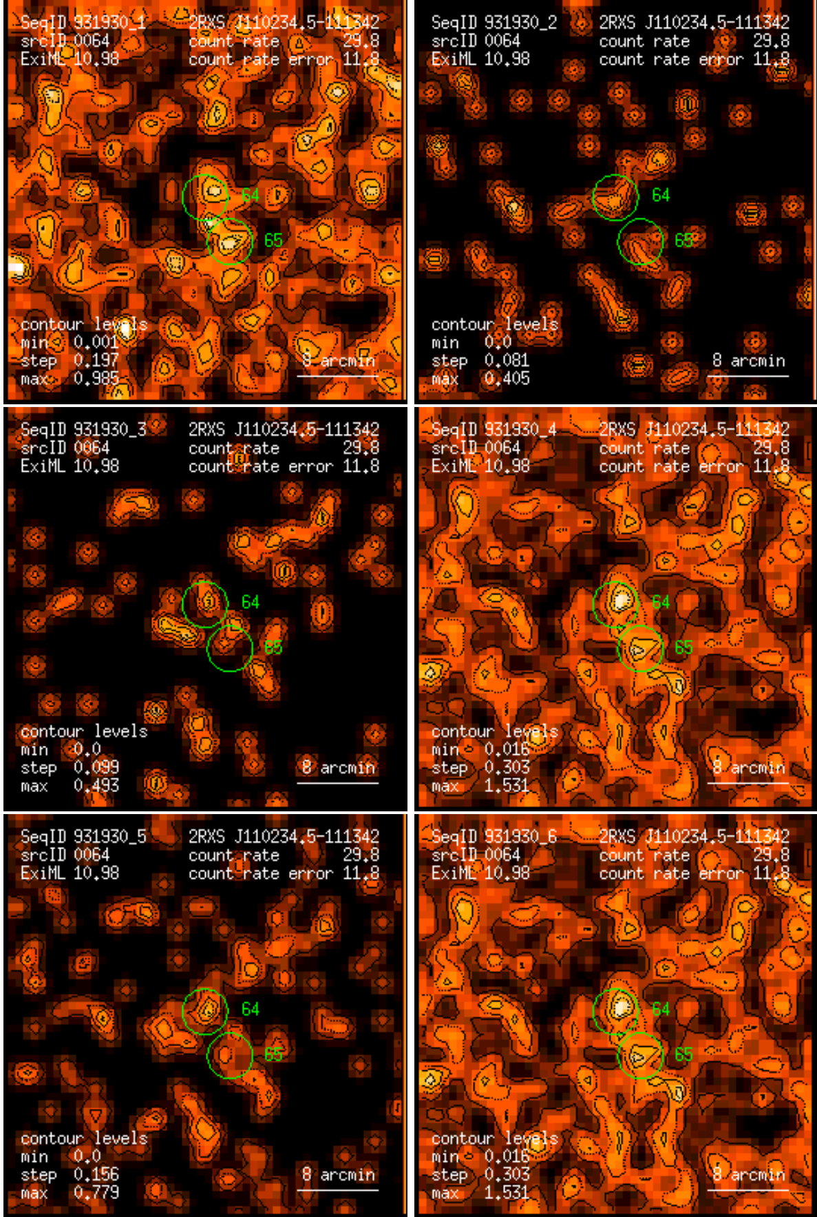
Figure 64: RASS 931930: detection 0064: band rate images, Gaussian filter: (1) PSPC channels 11 – 41, (2) 52 – 90, (3) 91 – 201, (4) 11 – 235, (5) 52 – 201, (6) 11 – 201. Broad band rates in counts/ks. Band rate contour levels in counts/ks/arcmin 2 .
