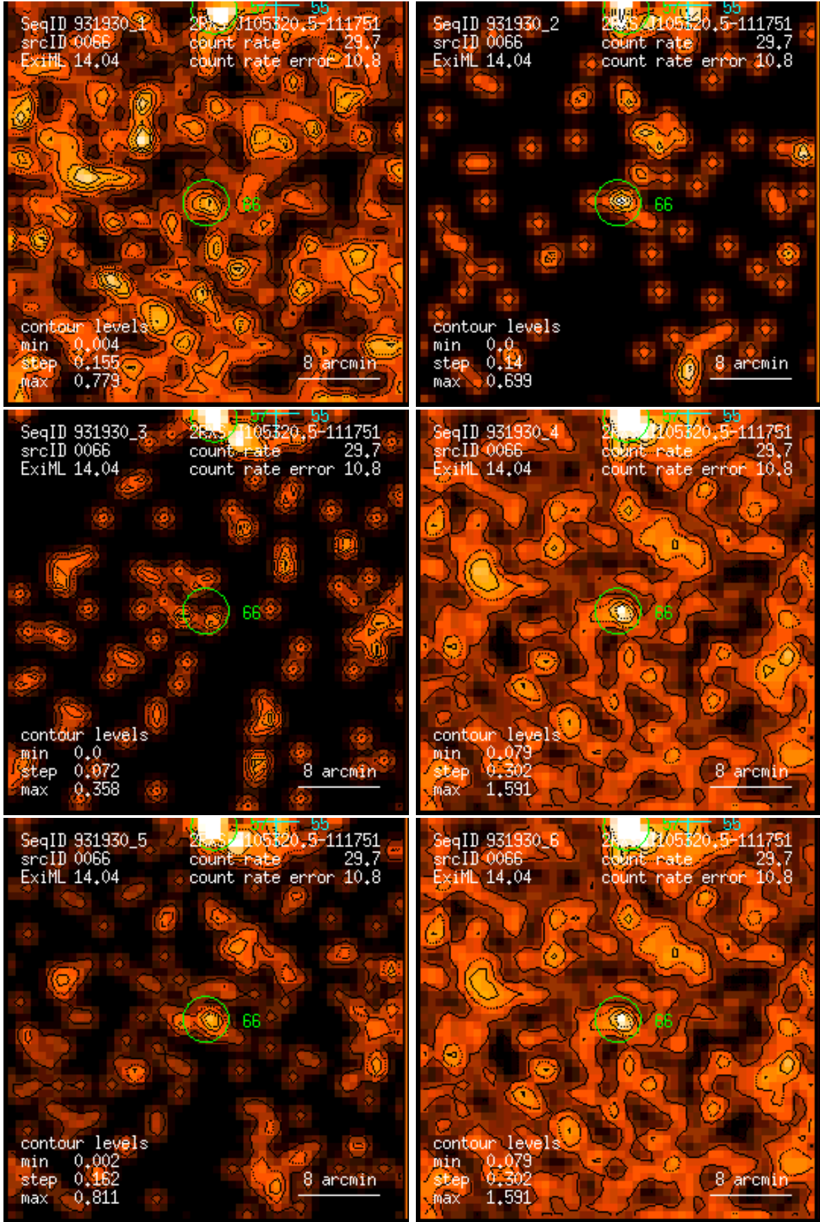
Figure 66: RASS 931930: detection 0066: band rate images, Gaussian filter: (1) PSPC channels 11 – 41, (2) 52 – 90, (3) 91 – 201, (4) 11 – 235, (5) 52 – 201, (6) 11 – 201. Broad band rates in counts/ks. Band rate contour levels in counts/ks/arcmin 2 .
