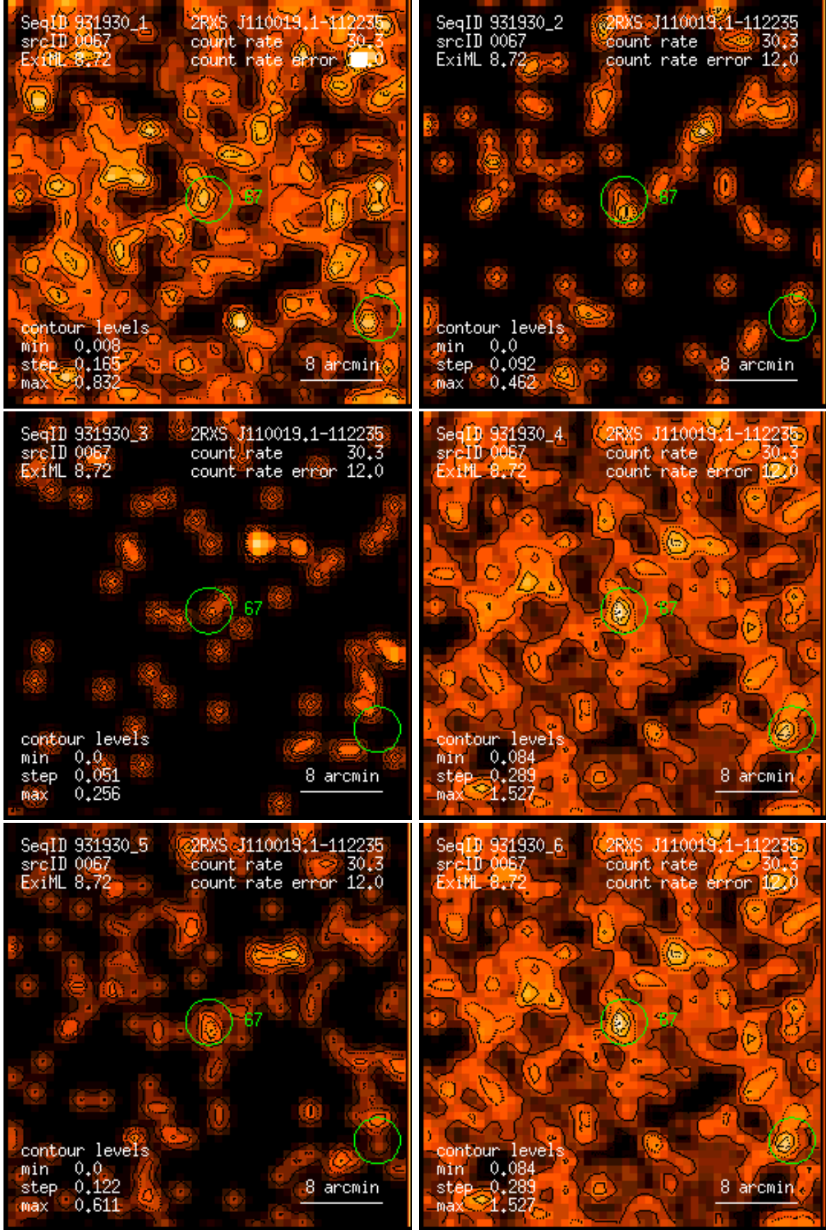
Figure 67: RASS 931930: detection 0067: band rate images, Gaussian filter: (1) PSPC channels 11 – 41, (2) 52 – 90, (3) 91 – 201, (4) 11 – 235, (5) 52 – 201, (6) 11 – 201. Broad band rates in counts/ks. Band rate contour levels in counts/ks/arcmin 2 .
