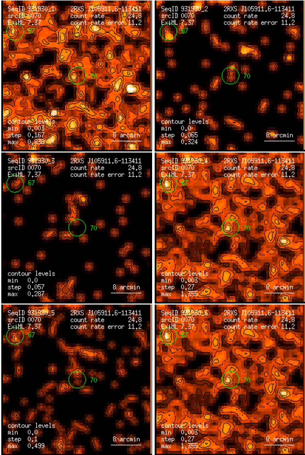
Figure 70: RASS 931930: detection 0070: band rate images, Gaussian filter: (1) PSPC channels 11 – 41, (2) 52 – 90, (3) 91 – 201, (4) 11 – 235, (5) 52 – 201, (6) 11 – 201. Broad band rates in counts/ks. Band rate contour levels in counts/ks/arcmin 2 .
