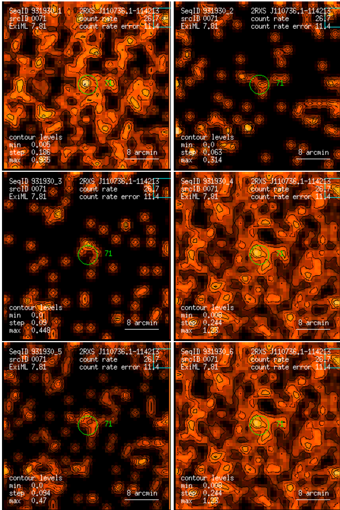
Figure 71: RASS 931930: detection 0071: band rate images, Gaussian filter: (1) PSPC channels 11 – 41, (2) 52 – 90, (3) 91 – 201, (4) 11 – 235, (5) 52 – 201, (6) 11 – 201. Broad band rates in counts/ks. Band rate contour levels in counts/ks/arcmin 2 .
