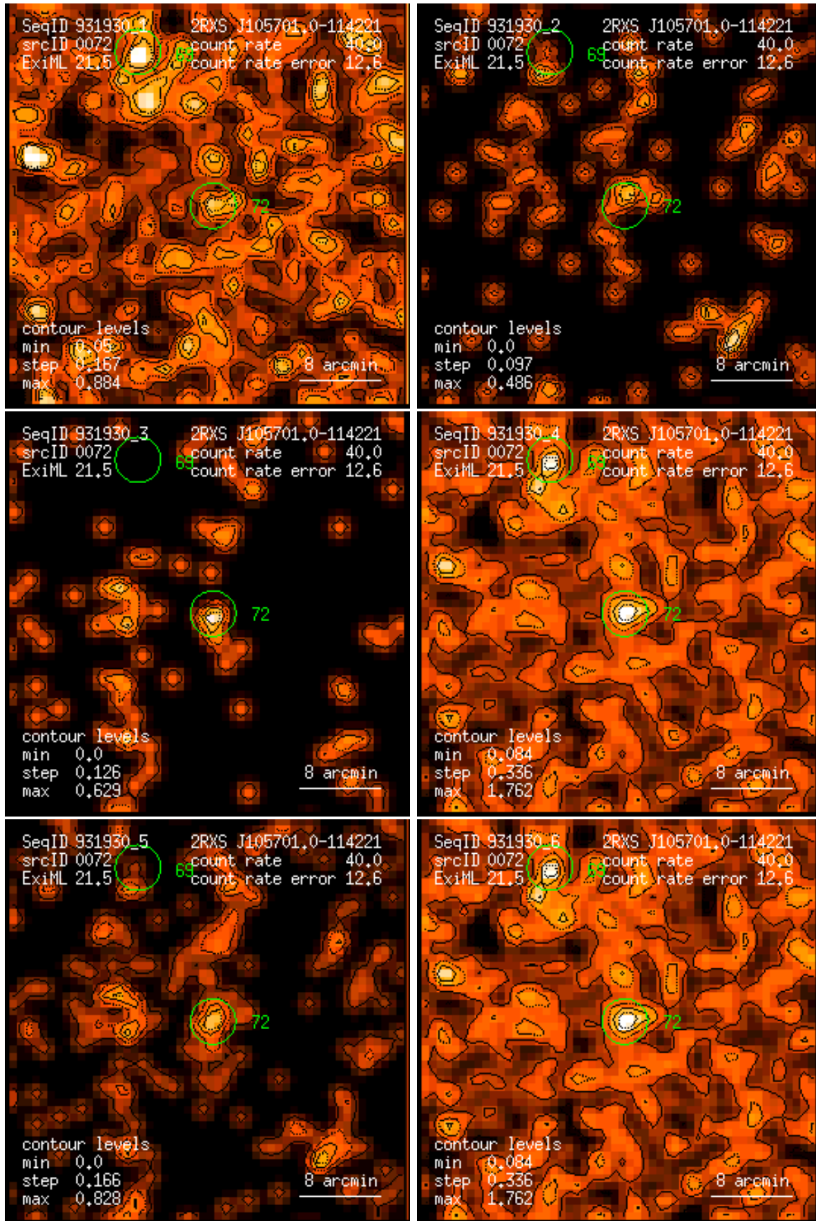
Figure 72: RASS 931930: detection 0072: band rate images, Gaussian filter: (1) PSPC channels 11 – 41, (2) 52 – 90, (3) 91 – 201, (4) 11 – 235, (5) 52 – 201, (6) 11 – 201. Broad band rates in counts/ks. Band rate contour levels in counts/ks/arcmin 2 .
