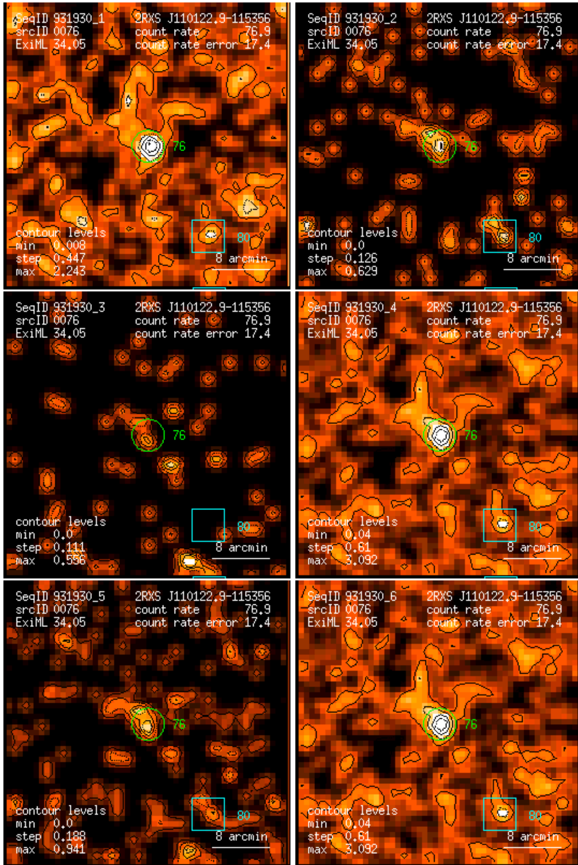
Figure 76: RASS 931930: detection 0076: band rate images, Gaussian filter: (1) PSPC channels 11 – 41, (2) 52 – 90, (3) 91 – 201, (4) 11 – 235, (5) 52 – 201, (6) 11 – 201. Broad band rates in counts/ks. Band rate contour levels in counts/ks/arcmin 2 .
