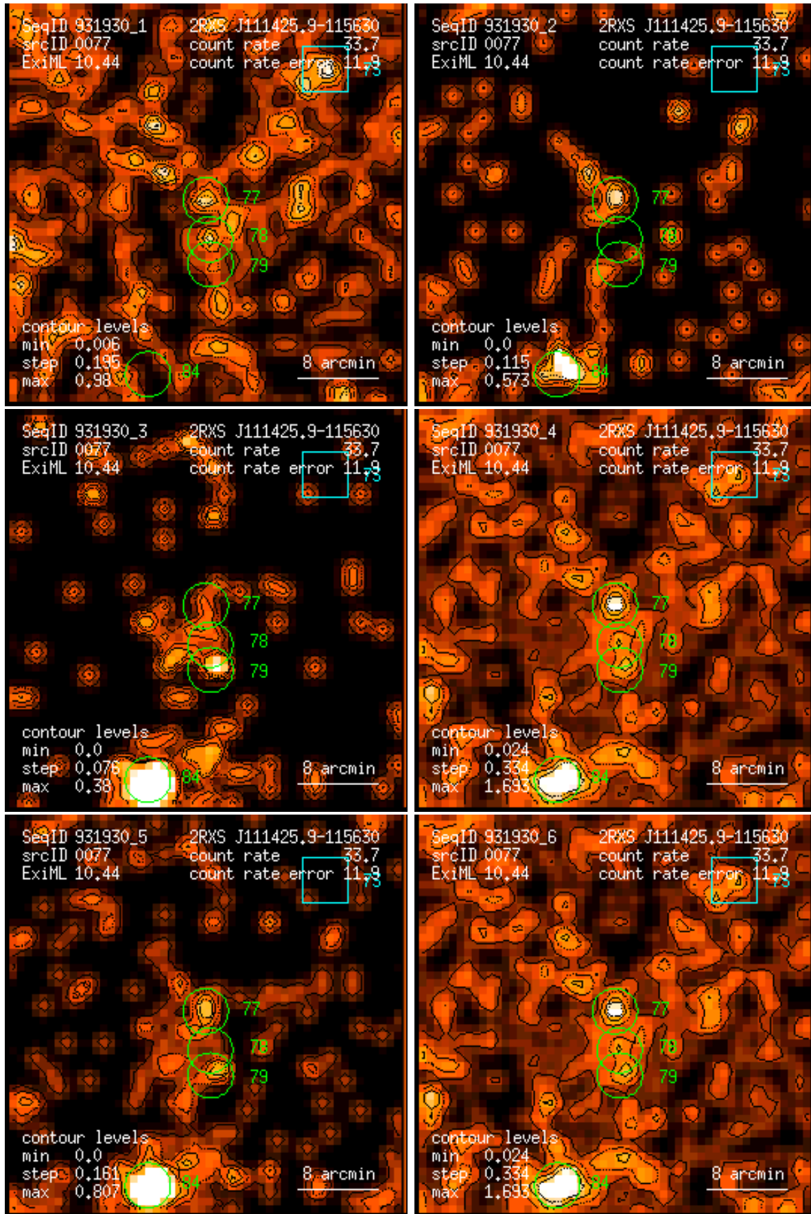
Figure 77: RASS 931930: detection 0077: band rate images, Gaussian filter: (1) PSPC channels 11 – 41, (2) 52 – 90, (3) 91 – 201, (4) 11 – 235, (5) 52 – 201, (6) 11 – 201. Broad band rates in counts/ks. Band rate contour levels in counts/ks/arcmin 2 .
