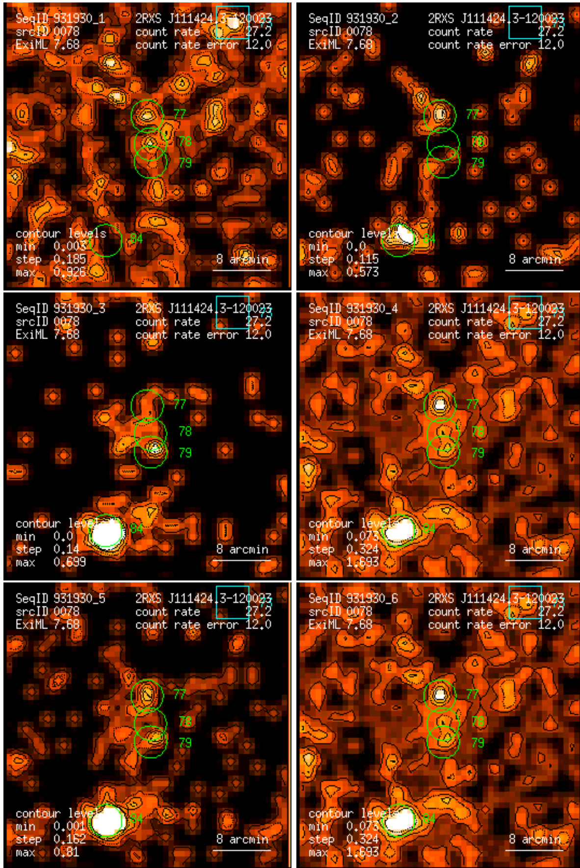
Figure 78: RASS 931930: detection 0078: band rate images, Gaussian filter: (1) PSPC channels 11 – 41, (2) 52 – 90, (3) 91 – 201, (4) 11 – 235, (5) 52 – 201, (6) 11 – 201. Broad band rates in counts/ks. Band rate contour levels in counts/ks/arcmin 2 .
