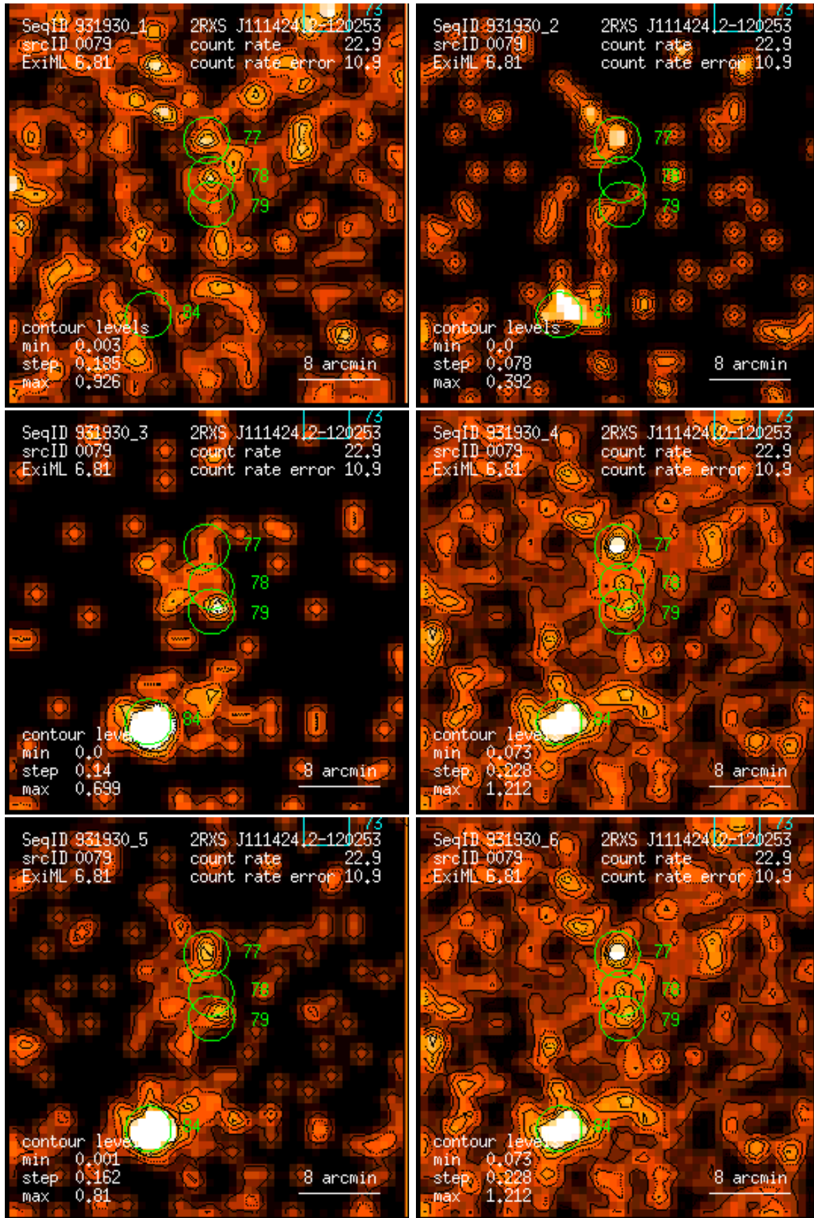
Figure 79: RASS 931930: detection 0079: band rate images, Gaussian filter: (1) PSPC channels 11 – 41, (2) 52 – 90, (3) 91 – 201, (4) 11 – 235, (5) 52 – 201, (6) 11 – 201. Broad band rates in counts/ks. Band rate contour levels in counts/ks/arcmin 2 .
