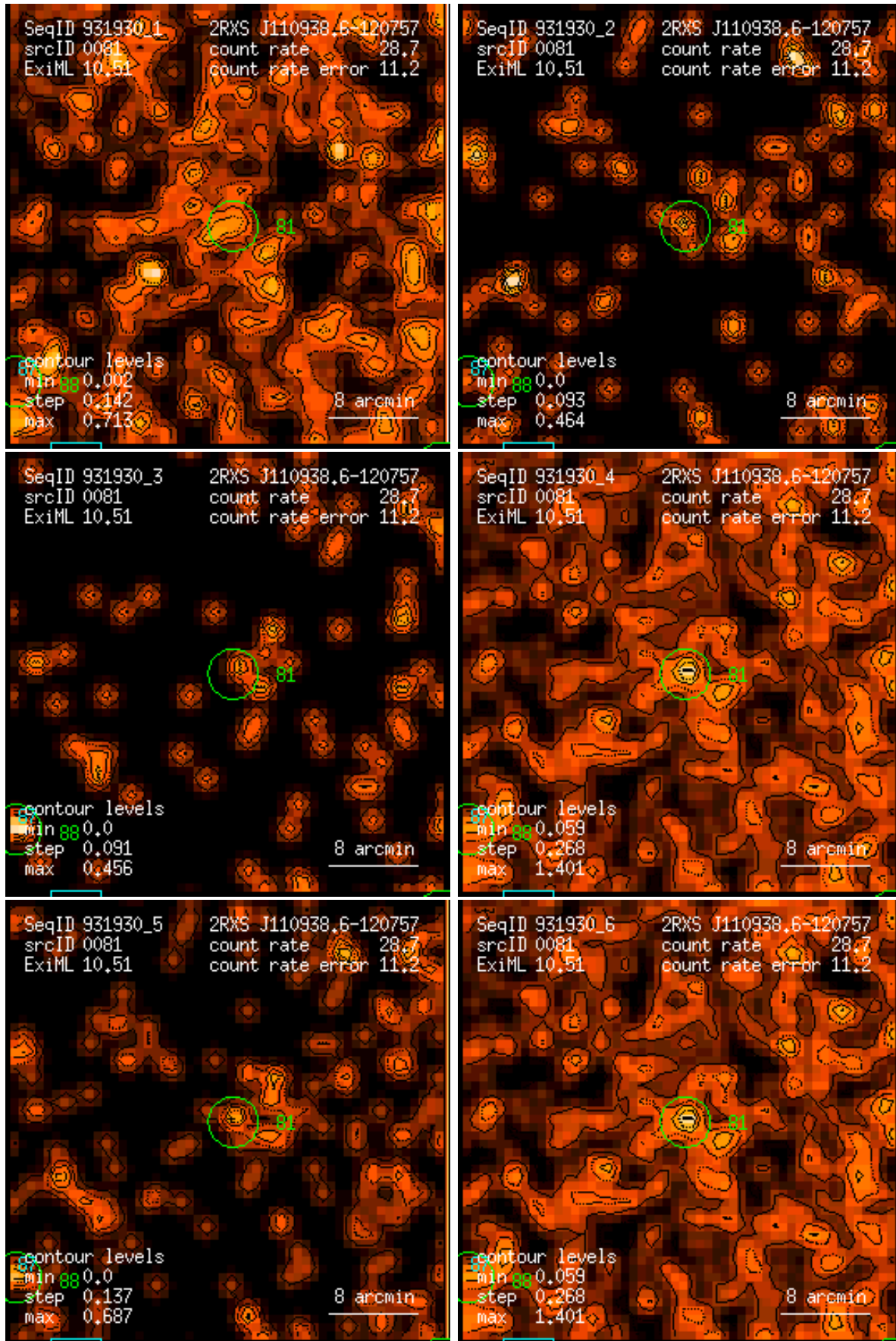
Figure 81: RASS 931930: detection 0081: band rate images, Gaussian filter: (1) PSPC channels 11 – 41, (2) 52 – 90, (3) 91 – 201, (4) 11 – 235, (5) 52 – 201, (6) 11 – 201. Broad band rates in counts/ks. Band rate contour levels in counts/ks/arcmin 2 .
