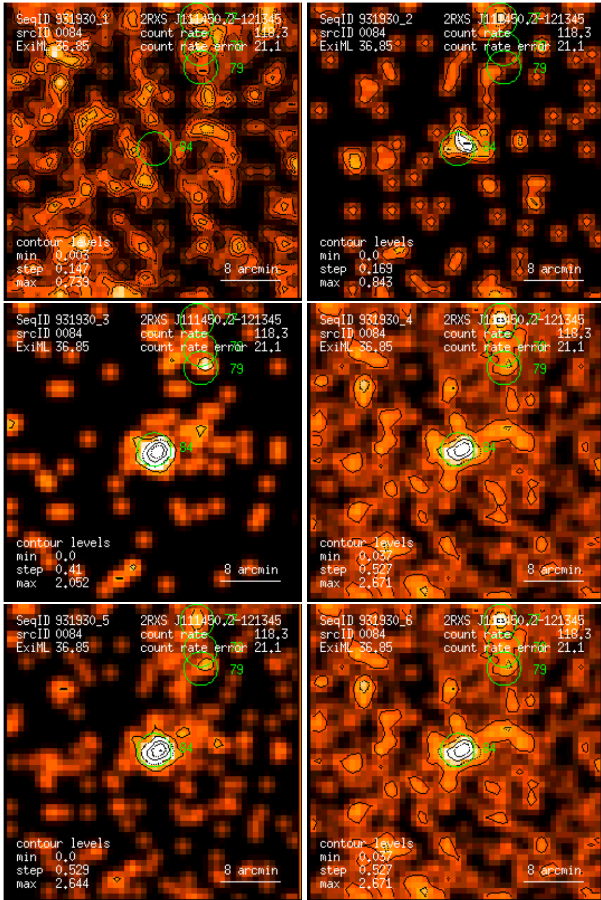
Figure 84: RASS 931930: detection 0084: band rate images, Gaussian filter: (1) PSPC channels 11 – 41, (2) 52 – 90, (3) 91 – 201, (4) 11 – 235, (5) 52 – 201, (6) 11 – 201. Broad band rates in counts/ks. Band rate contour levels in counts/ks/arcmin 2 .
