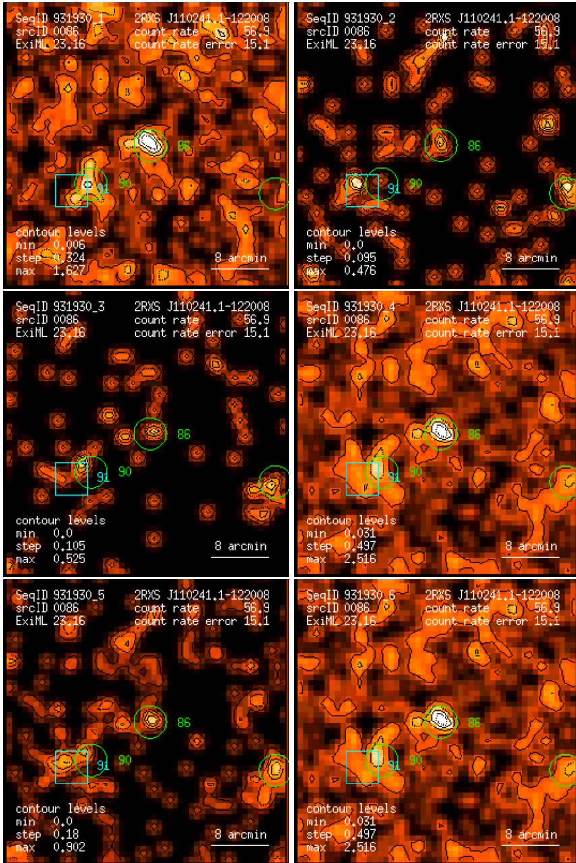
Figure 86: RASS 931930: detection 0086: band rate images, Gaussian filter: (1) PSPC channels 11 – 41, (2) 52 – 90, (3) 91 – 201, (4) 11 – 235, (5) 52 – 201, (6) 11 – 201. Broad band rates in counts/ks. Band rate contour levels in counts/ks/arcmin 2 .
