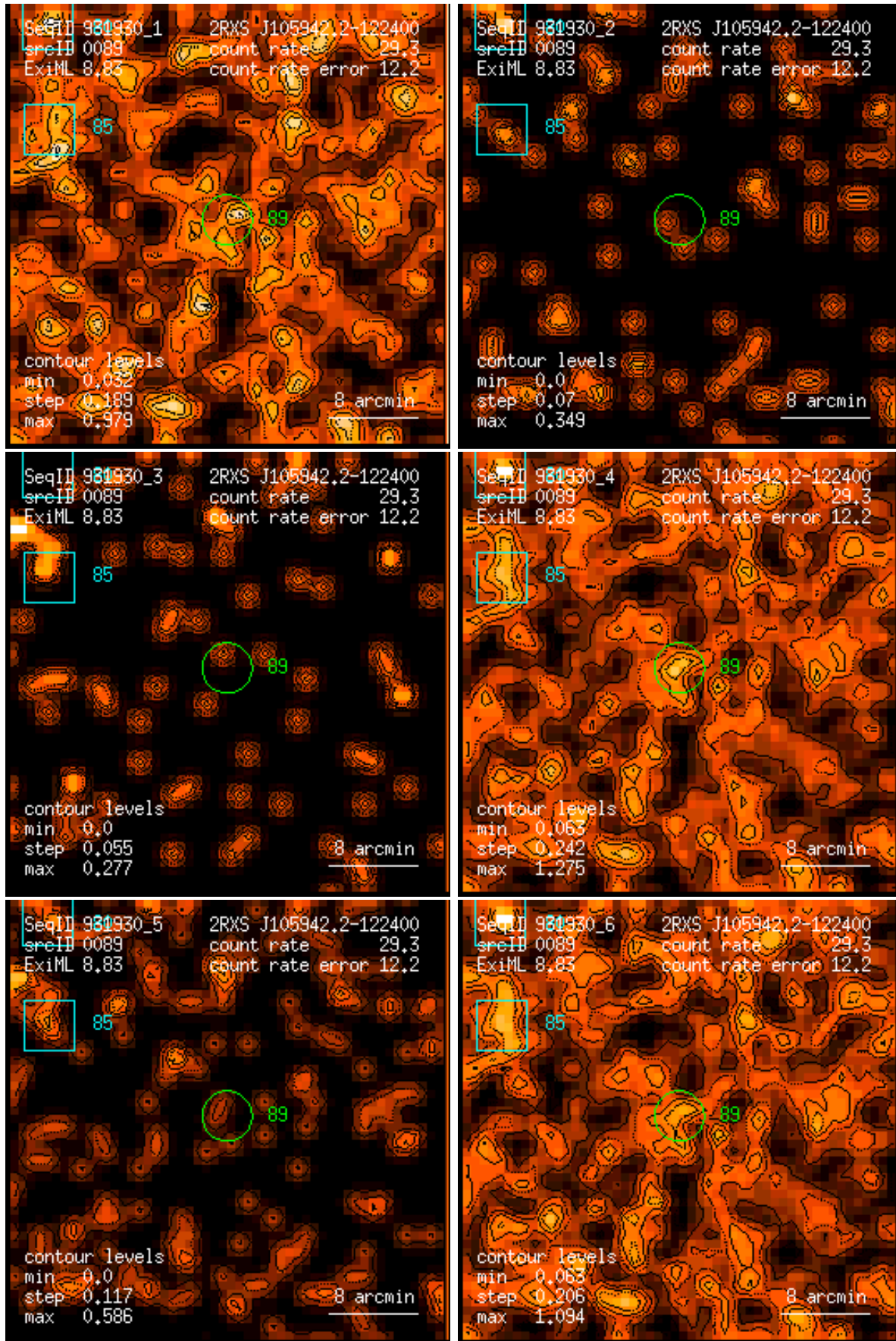
Figure 89: RASS 931930: detection 0089: band rate images, Gaussian filter: (1) PSPC channels 11 – 41, (2) 52 – 90, (3) 91 – 201, (4) 11 – 235, (5) 52 – 201, (6) 11 – 201. Broad band rates in counts/ks. Band rate contour levels in counts/ks/arcmin 2 .
