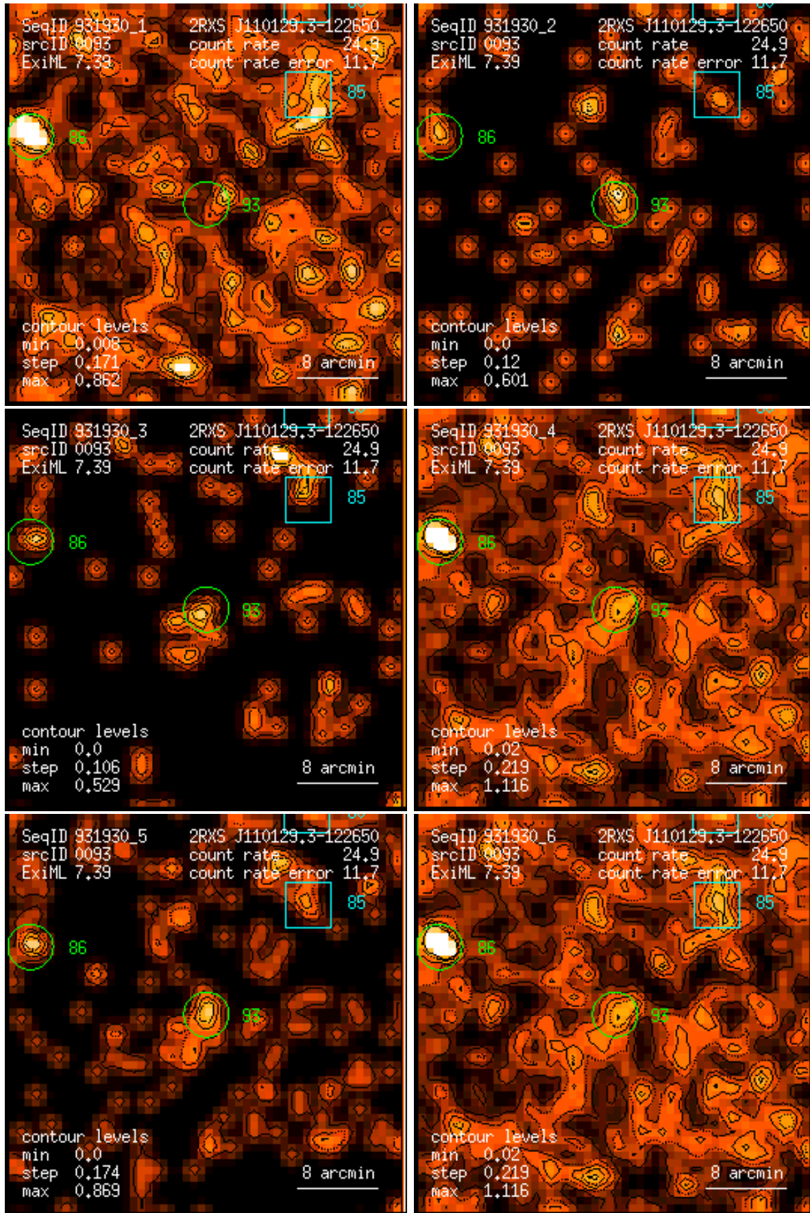
Figure 93: RASS 931930: detection 0093: band rate images, Gaussian filter: (1) PSPC channels 11 – 41, (2) 52 – 90, (3) 91 – 201, (4) 11 – 235, (5) 52 – 201, (6) 11 – 201. Broad band rates in counts/ks. Band rate contour levels in counts/ks/arcmin 2 .
