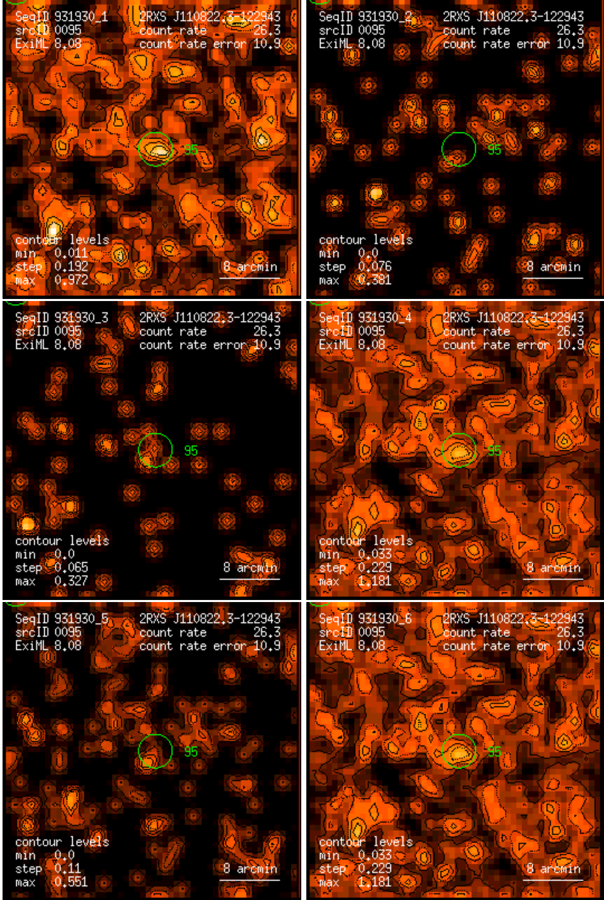
Figure 95: RASS 931930: detection 0095: band rate images, Gaussian filter: (1) PSPC channels 11 – 41, (2) 52 – 90, (3) 91 – 201, (4) 11 – 235, (5) 52 – 201, (6) 11 – 201. Broad band rates in counts/ks. Band rate contour levels in counts/ks/arcmin 2 .
