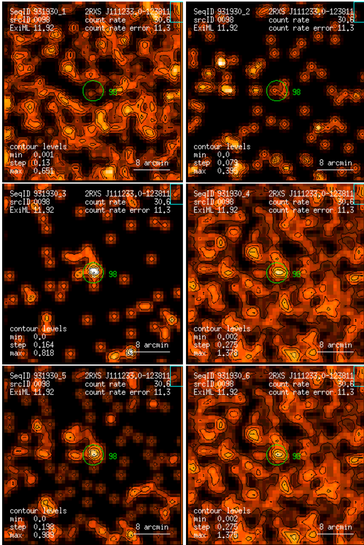
Figure 98: RASS 931930: detection 0098: band rate images, Gaussian filter: (1) PSPC channels 11 – 41, (2) 52 – 90, (3) 91 – 201, (4) 11 – 235, (5) 52 – 201, (6) 11 – 201. Broad band rates in counts/ks. Band rate contour levels in counts/ks/arcmin 2 .
