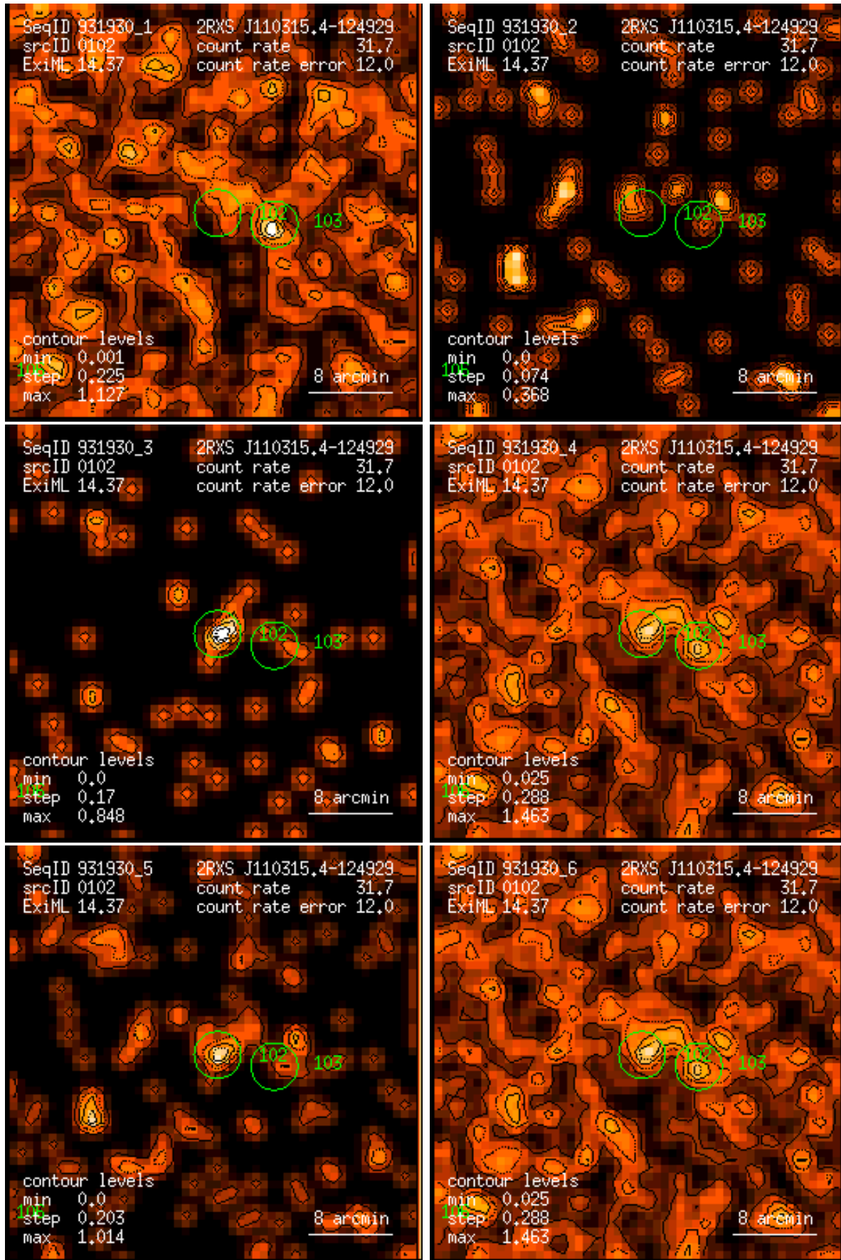
Figure 102: RASS 931930: detection 0102: band rate images, Gaussian filter: (1) PSPC channels 11 – 41, (2) 52 – 90, (3) 91 – 201, (4) 11 – 235, (5) 52 – 201, (6) 11 – 201. Broad band rates in counts/ks. Band rate contour levels in counts/ks/arcmin 2 .
