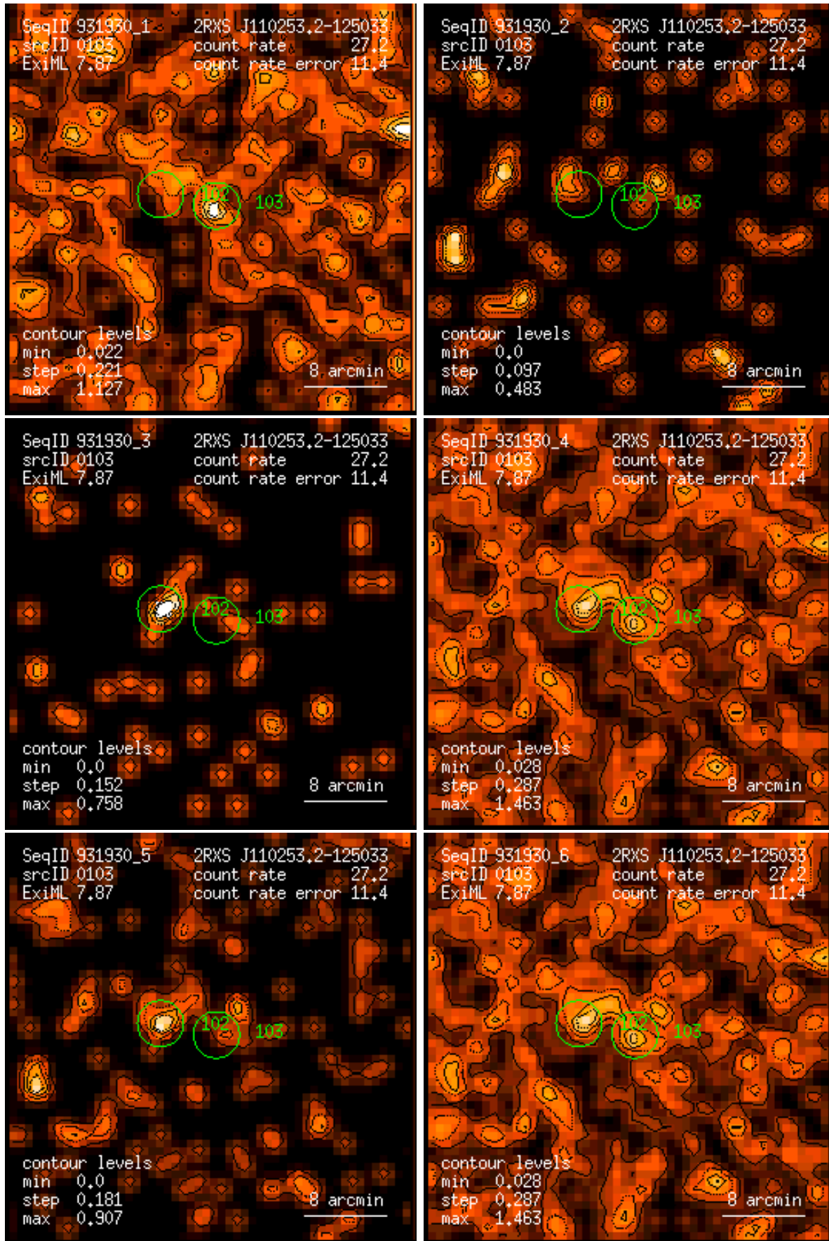
Figure 103: RASS 931930: detection 0103: band rate images, Gaussian filter: (1) PSPC channels 11 – 41, (2) 52 – 90, (3) 91 – 201, (4) 11 – 235, (5) 52 – 201, (6) 11 – 201. Broad band rates in counts/ks. Band rate contour levels in counts/ks/arcmin 2 .
