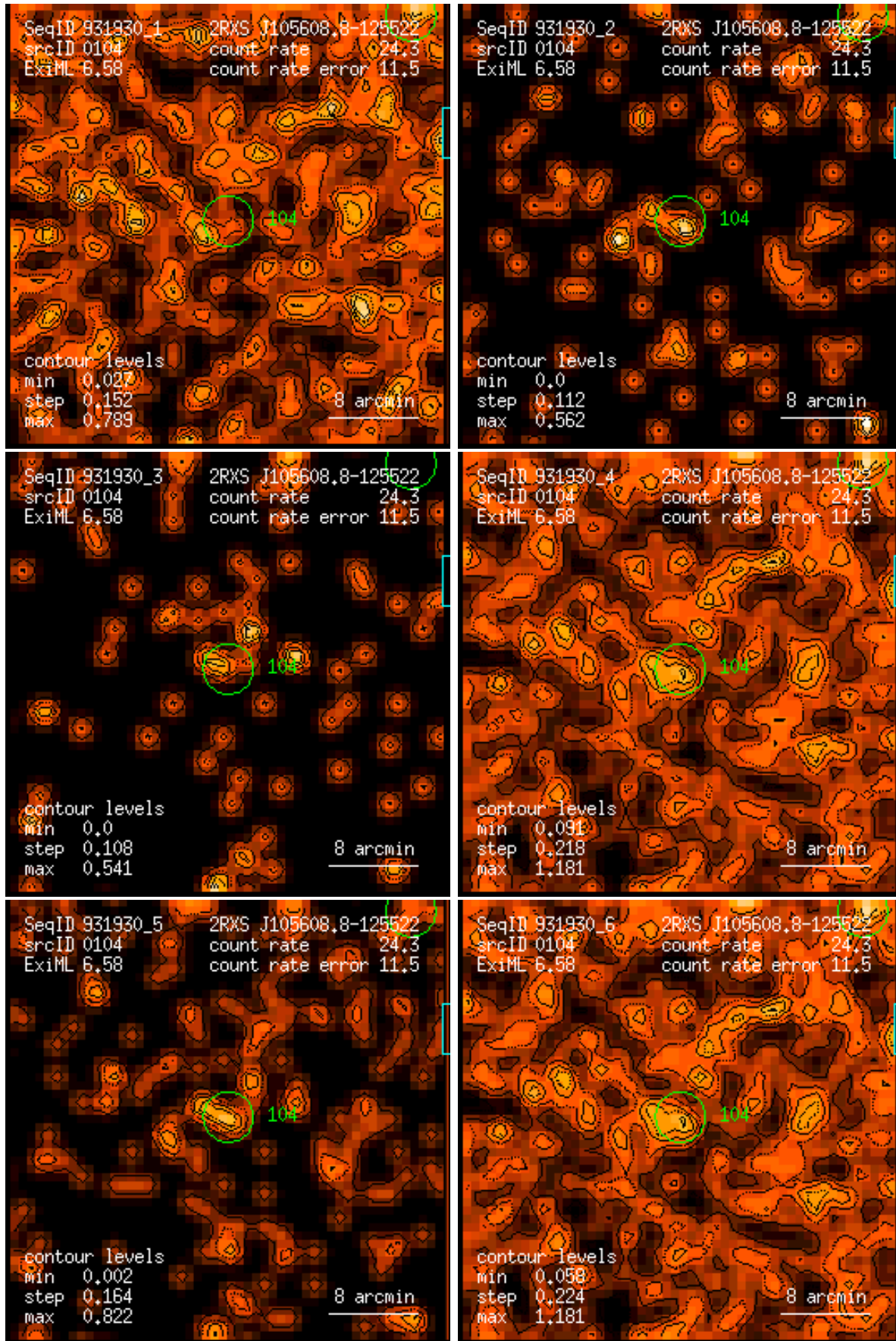
Figure 104: RASS 931930: detection 0104: band rate images, Gaussian filter: (1) PSPC channels 11 – 41, (2) 52 – 90, (3) 91 – 201, (4) 11 – 235, (5) 52 – 201, (6) 11 – 201. Broad band rates in counts/ks. Band rate contour levels in counts/ks/arcmin 2 .
