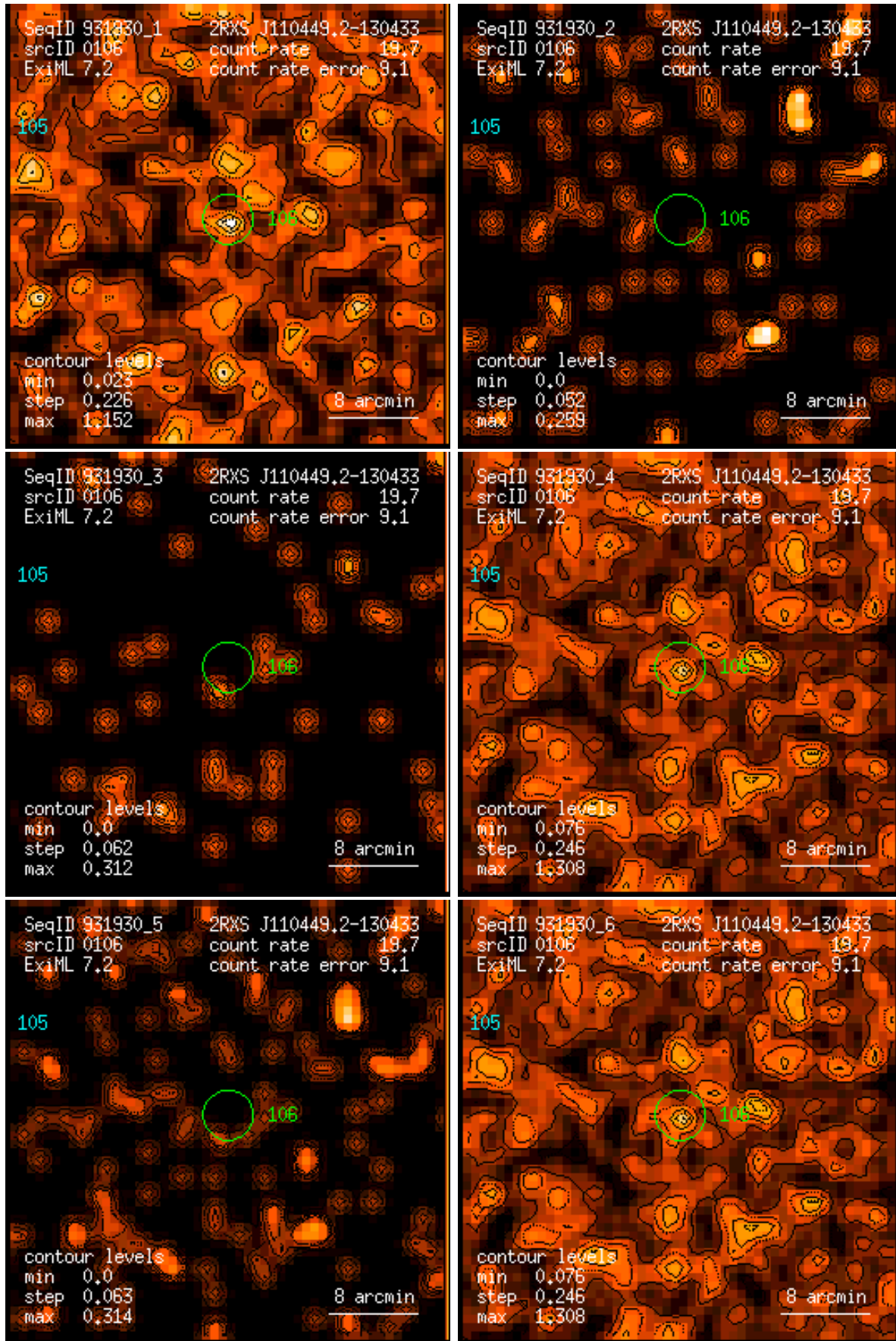
Figure 106: RASS 931930: detection 0106: band rate images, Gaussian filter: (1) PSPC channels 11 – 41, (2) 52 – 90, (3) 91 – 201, (4) 11 – 235, (5) 52 – 201, (6) 11 – 201. Broad band rates in counts/ks. Band rate contour levels in counts/ks/arcmin 2 .
